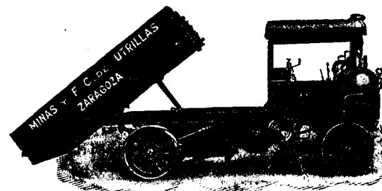
Tipping Wagon with Patent Mechanically-operated Tipping Gear.
