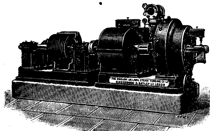
No. 6412. DE LAVAL PATENT STEAM TURBINE MOTOR. Type M.M.T. 225 B.H.P.
