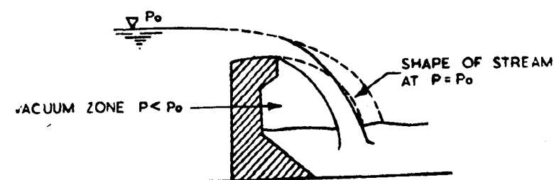
FIG. 3 FREE FALLING STREAM.
