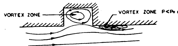
FIG 2 GATE SLOTS.
