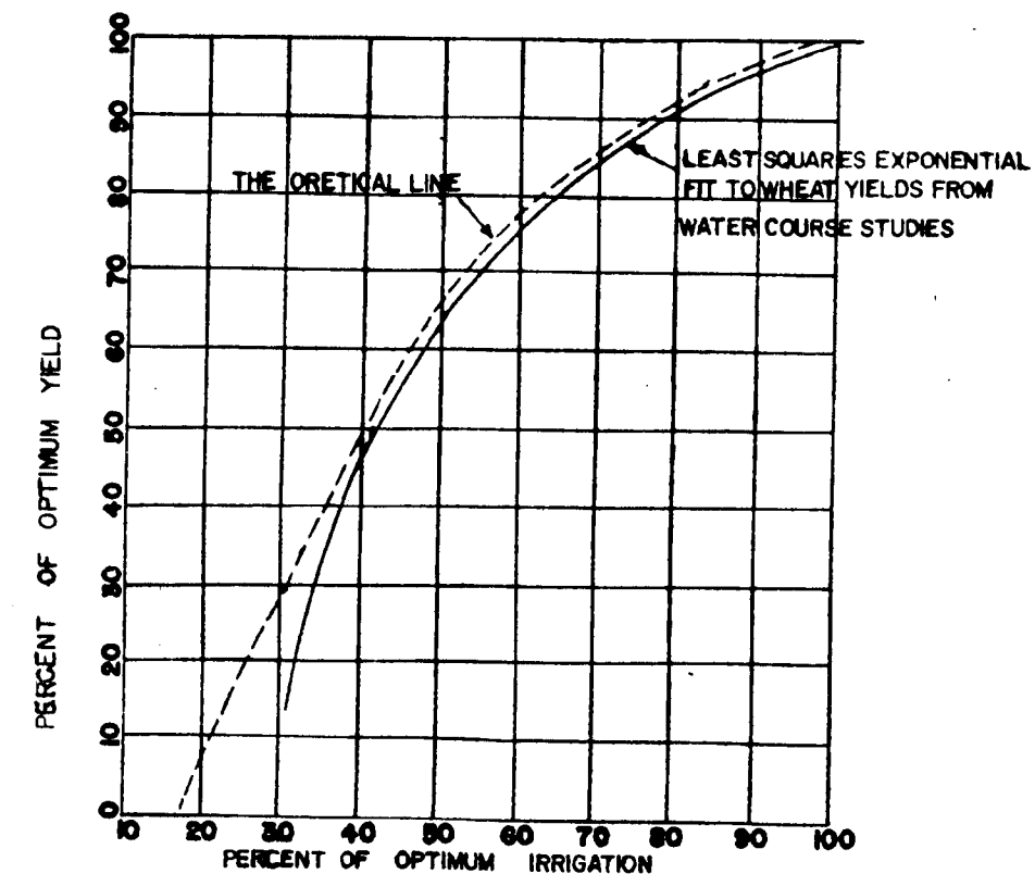
RELATIONSHIP BETWEEN YIELD & IRRIGATION
