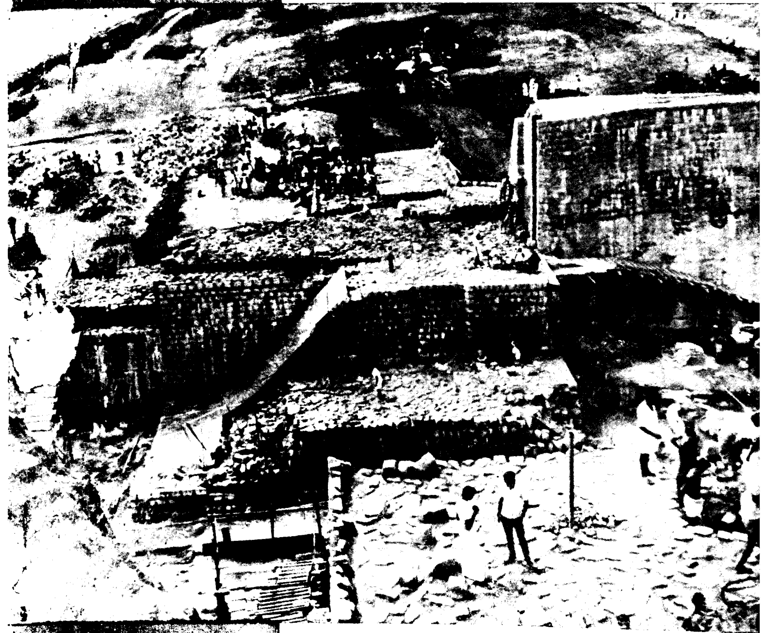
Ponmaniar Project—Masonry Dam in Progress.
