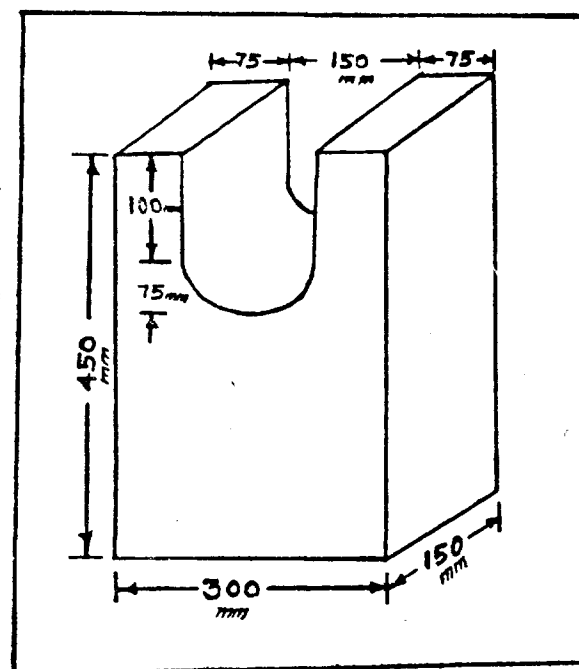
Head-piece
