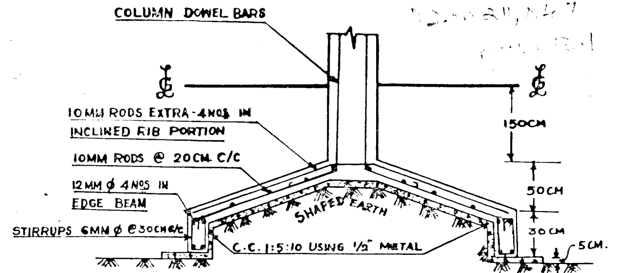
SECTION
