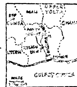
KOSSOU DAM 4-mile-long rockfill is located 186 miles from the coast.
