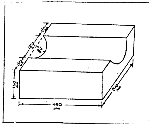
Drain-piece
