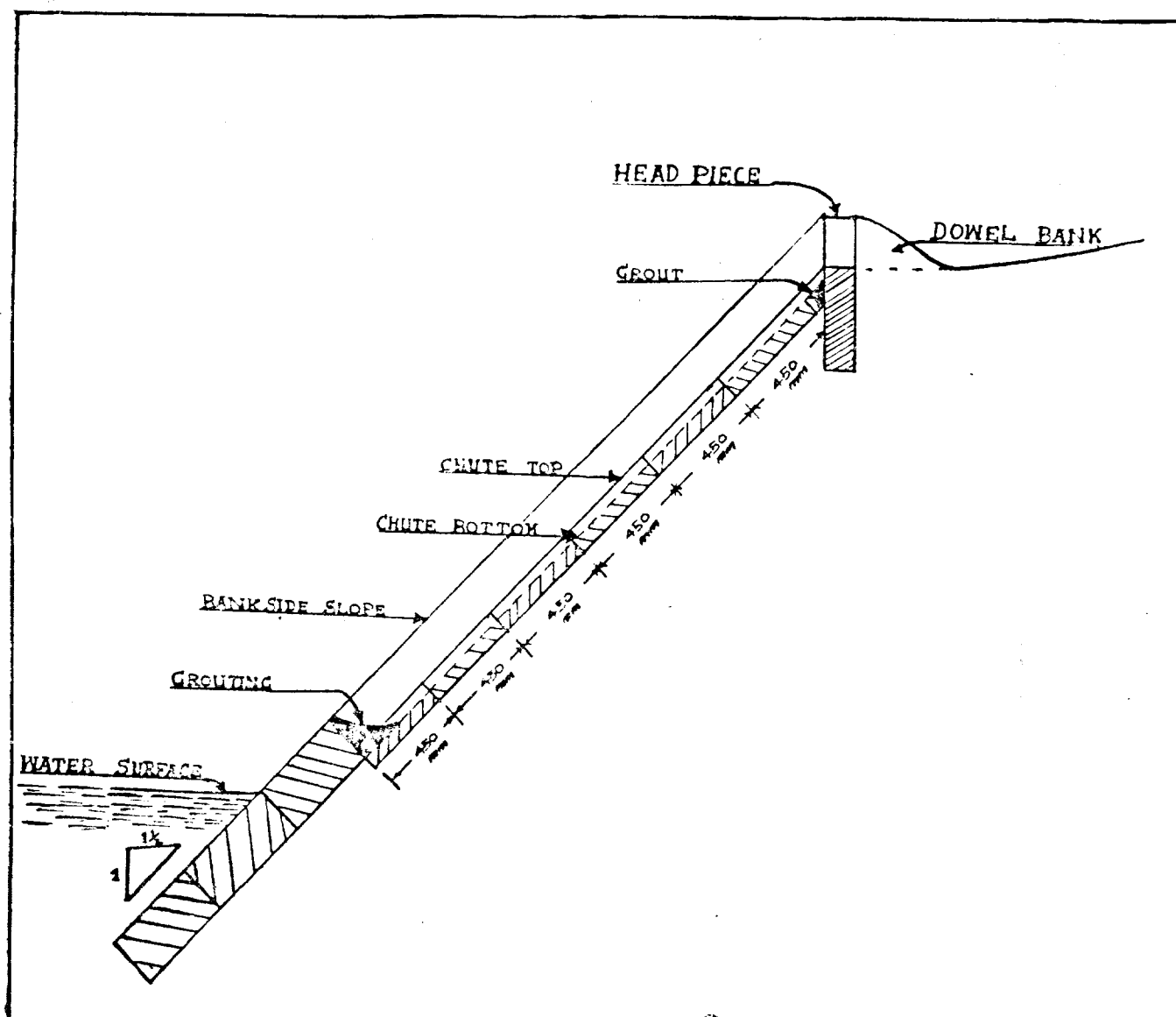
Drain-piece
