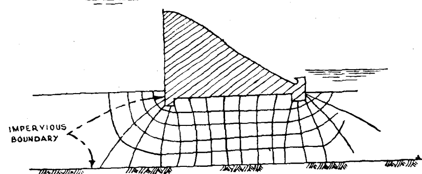
FLOW NET UNDER A WEIR ON PVIOUS FOUNDATION SKETCH.1
