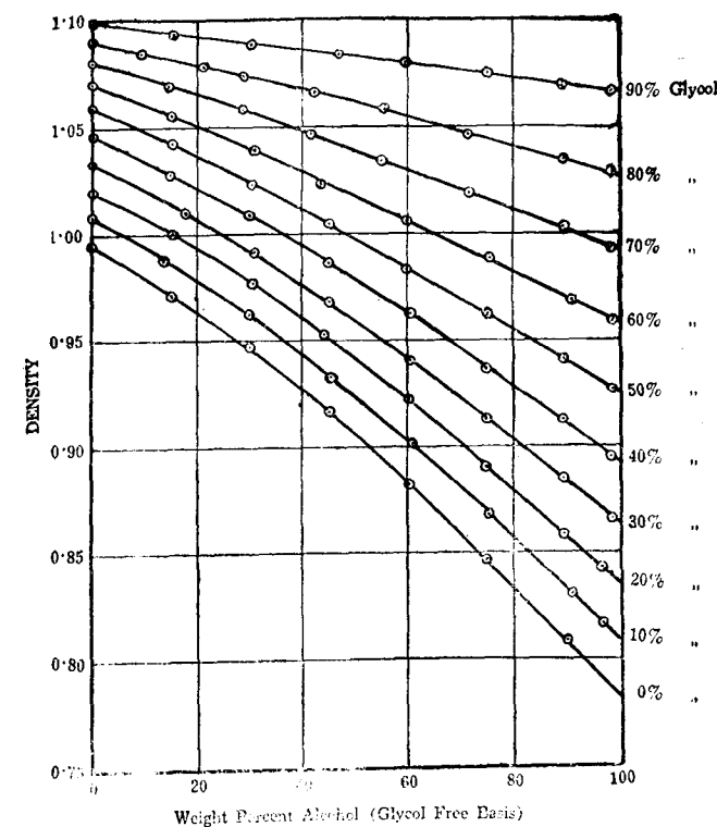
FIG. 1. Density — Composition Diagram
