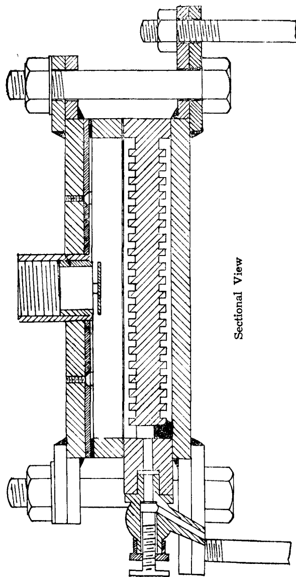
Fig. 2. Filter for slow filtering slurries.
