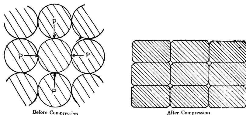
FIG. 6. Effect of pressure on compressible particles.
