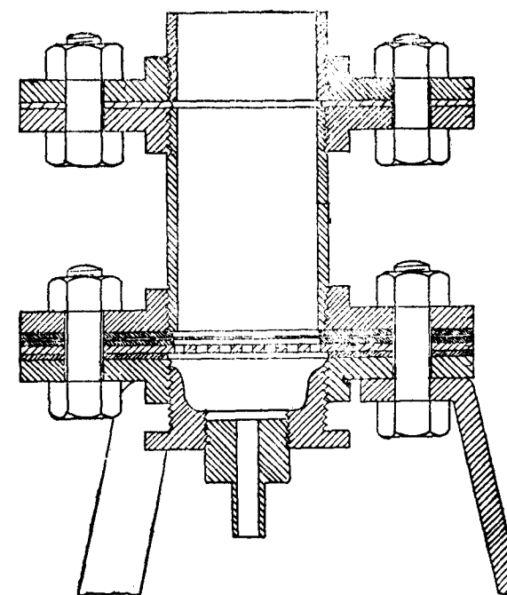
FIG. 1. Filter for fast filtering Slurries.
