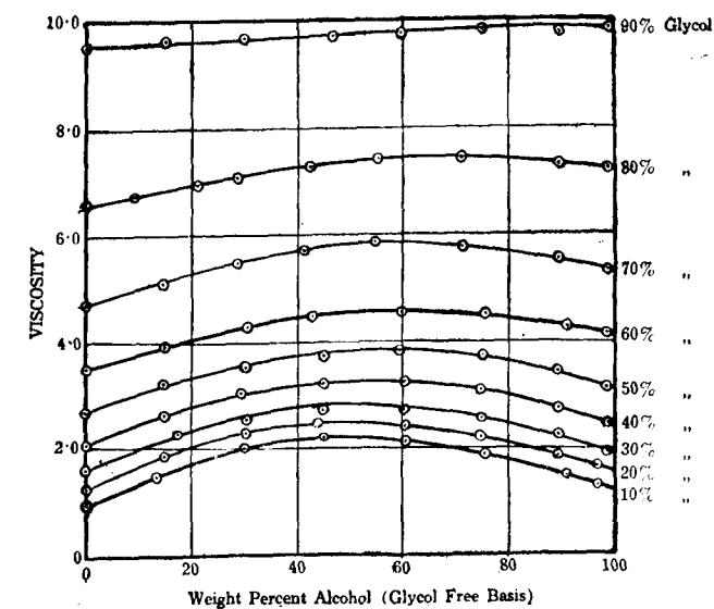
FIG. 2. Viscosity — Composition Diagram
