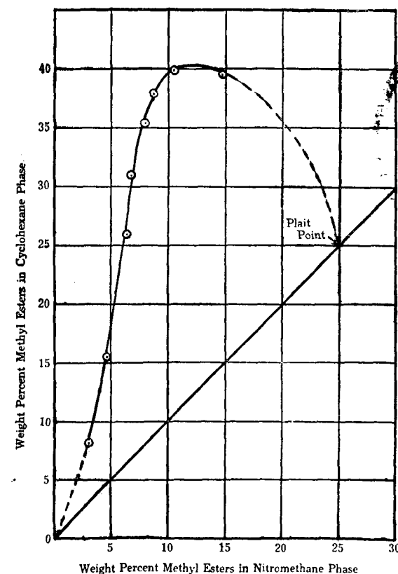
FIG. 2. Equilibrium Distribution Diagram.
