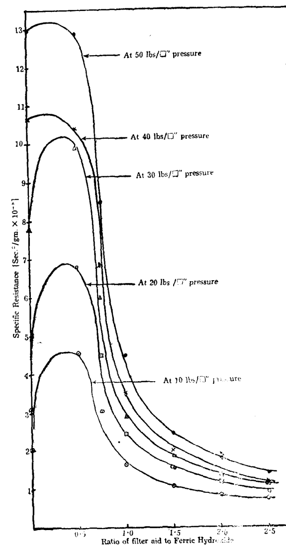
FIG. 4. Experiments with Filtercel.
