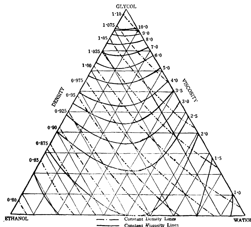
FIG. 3. Density and Viscosity of Ethanol. Water—Ethylene Glycol system.
