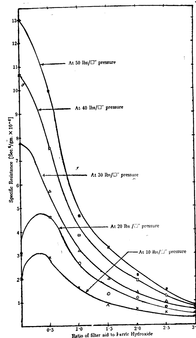
FIG. 5. Experiments with Hiflo Supercel
