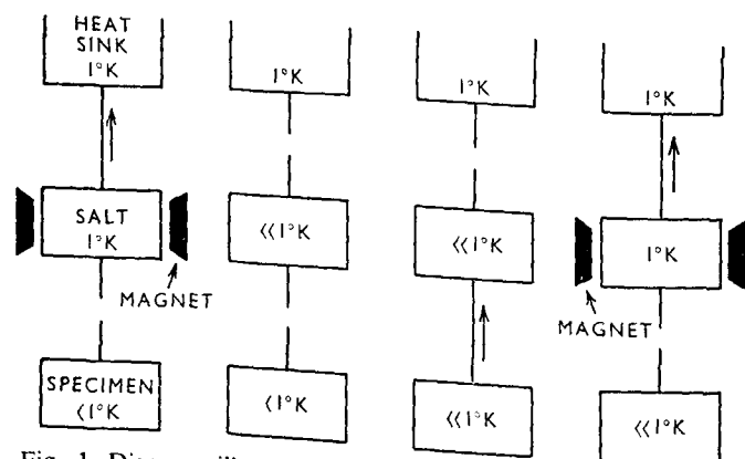
Fig. 1. Diagram illustrating the operation of Daunt's magnetic refrigerator. The arrows indicate the direction of the heat flow and a break in the connecting lines means that the thermal switch is superconductive.
