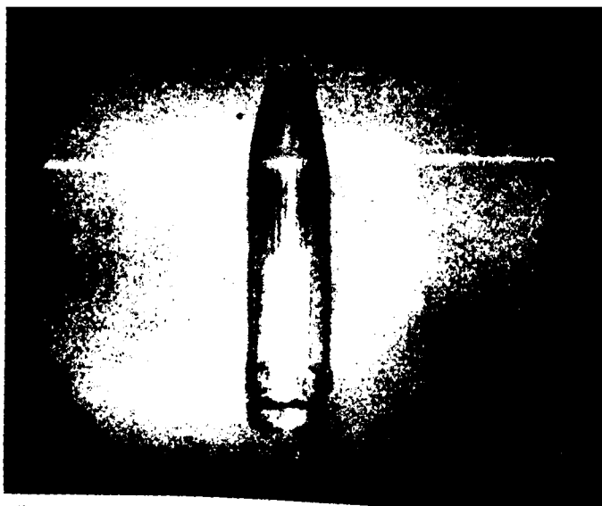
17. Bullet travelling at 2,400 ft/sec. photographed with image converter equipment: exposure time 1 \mu sec.
