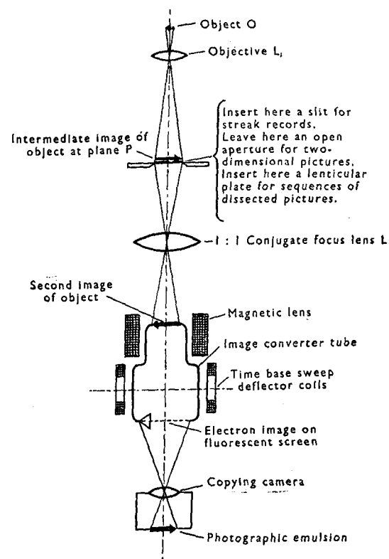
Fig. 2. Schematic diagram of image converter tube apparatus with an intermediate image plane at P. If a slit is placed at P this apparatus can be used for streak records. If an open aperture is left at P the apparatus can take ordinary two-dimensional pictures of very short exposure. If a lenticular plate is placed at P the image at the photo-cathode is dissected into small dot elements. If a time sweep is then applied to the tube the composite dissected picture sequence appears on the fluorescent screen and can be recorded by a plate camera. The individual pictures of the sequence can subsequently be unscrambled. (Courtesy of Butterworth's Scientific Publications.)
