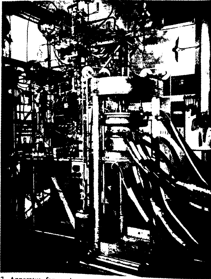
7. Apparatus for nuclear cooling. The water-cooled solenoid surrounding the cryostat produces the high magnetic field needed to align the atomic nuclei at 0.01^{\circ}\text{K} .
