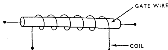
Fig. 2. Diagrammatic representation of a cryotron.
