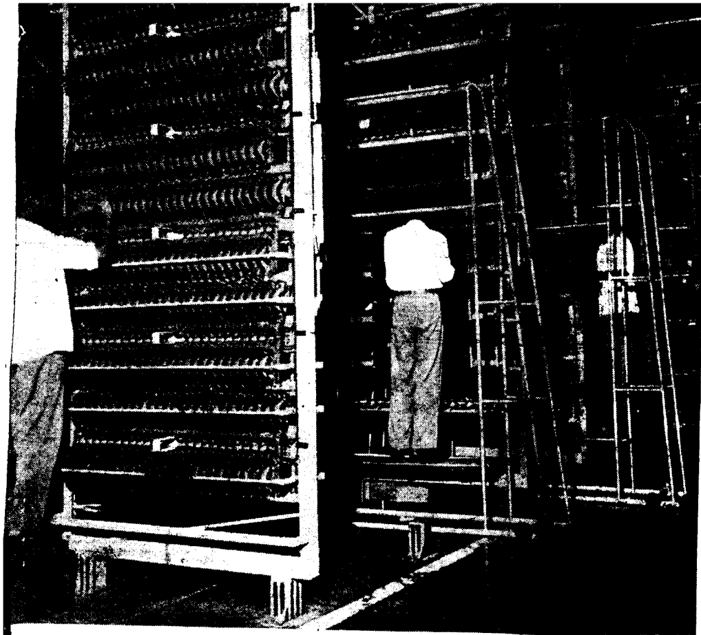
Assembly of wheels and body at one of the workshop sheds of the Integral Coach Factory at Perambur (Madras). In its first year ending October 1956 the Factory produced 43 unfinished coach shells whereas in its third year ending October 1958 the production rose to 300 shells
