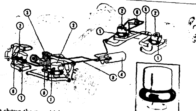
Photo above shows the new Airide Suspension system developed by the Firestone Tyre & Rubber Co. Compressed air, regulated by special leveling valves is forced into the bellows chamber to compensate for heavy loads, are allowed to escape in the case of lighter loads
