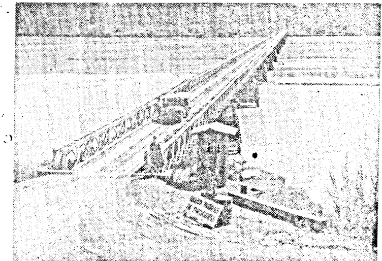
The largest bridge in New Guinea is the 1690-foot, single-span structure crossing the Markham River. Completed in 1955, it has made possible transit of heavy motor transports
