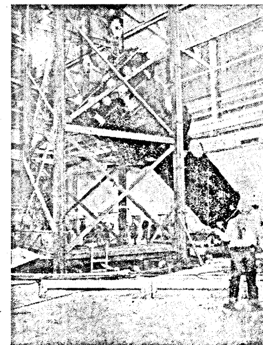
During construction of the Engineering Test Reactor the reactor vessel—"heart" of the new device—is raised to near vertical position for lowering into its receptacle
