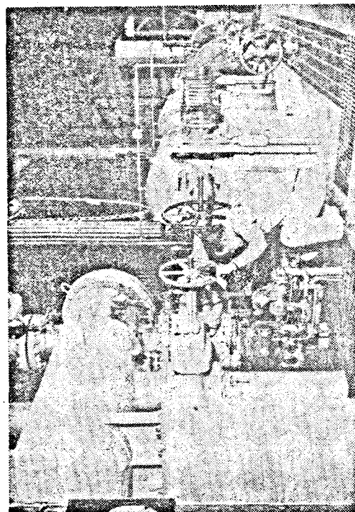
Workmen lower the grid plate into the 35-foot-deep pressure vessel of the Engineering Test Reactor
