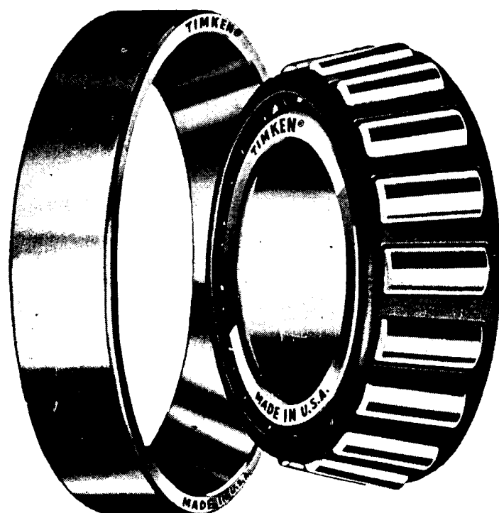
(1) This is the standard, single-row Timken (Made in U.S.A.) tapered roller bearing showing the cup, or outer race, on the left and the cone, rollers and cage on the right.
