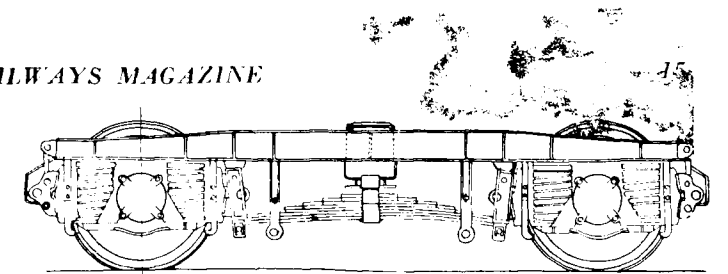
FIG-4 BOGIE OF SCHLIEREN COACH
