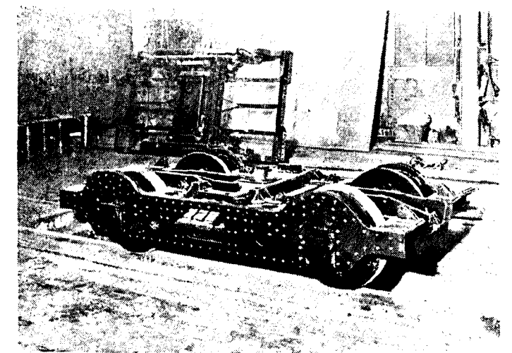
Fig. 3. A bogie showing the laminated elliptic springs under the bolster.
