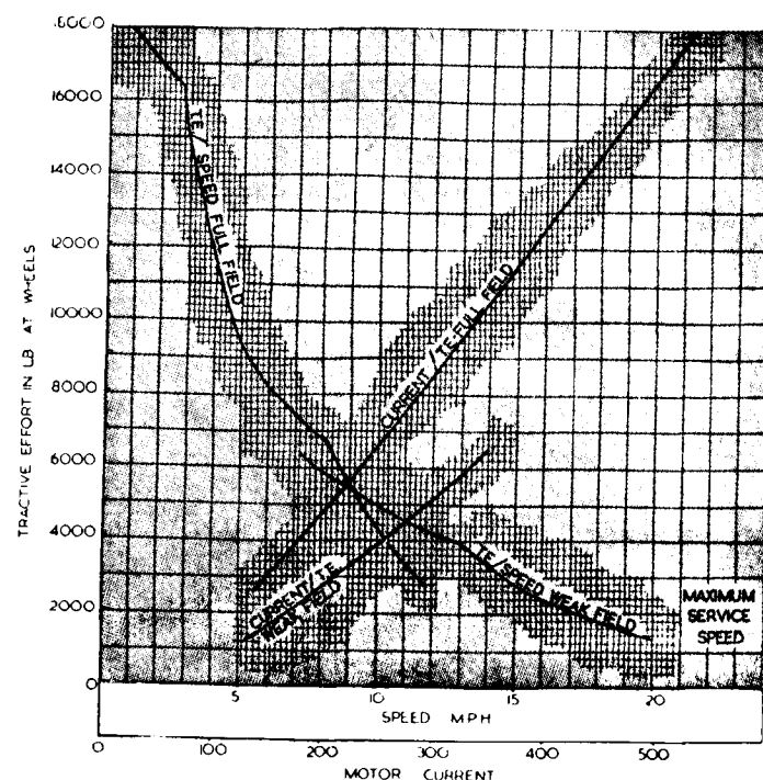
TRACTION EFFORT - SPEED CURVE
