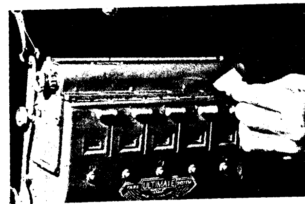
The five-unit version of the Ultimate machine, with a ticket being torn off. Tickets are issued by depressing the knobs located between the ticket apertures and the dials recording the number of issues.
