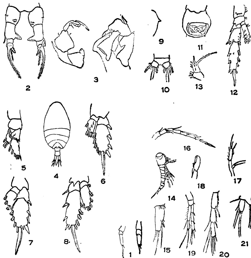
FIG. 1. Calocalanus plumoloses male fifth leg ( \times 400 ). FIGS. 2-3. Schmackeria tollingarae . Fifth leg female, (2), male (3), ( \times 280 ). FIGS. 4-8. Scolecithrix danae (4), Dorsal view ( \times 80 ), 1 to 4 ( \times 280 ). FIGS. 9-13. Scolecithricella ctenopus . Lateral view of the last thoracic segment, ( \times 280 ), (10) caudal ramus, (11) genital segment, (12) fourth leg, (13) fifth leg ( \times 400 ). FIG. 14-21. Miracia minor . Lateral view (14), caudal ramus (15), Antennule (16), Antenna (17), Maxillipede (18), first leg, (19) Exopod of second leg (20), fifth leg (21). All the appendages drawn to a magnification of \times 400 .
