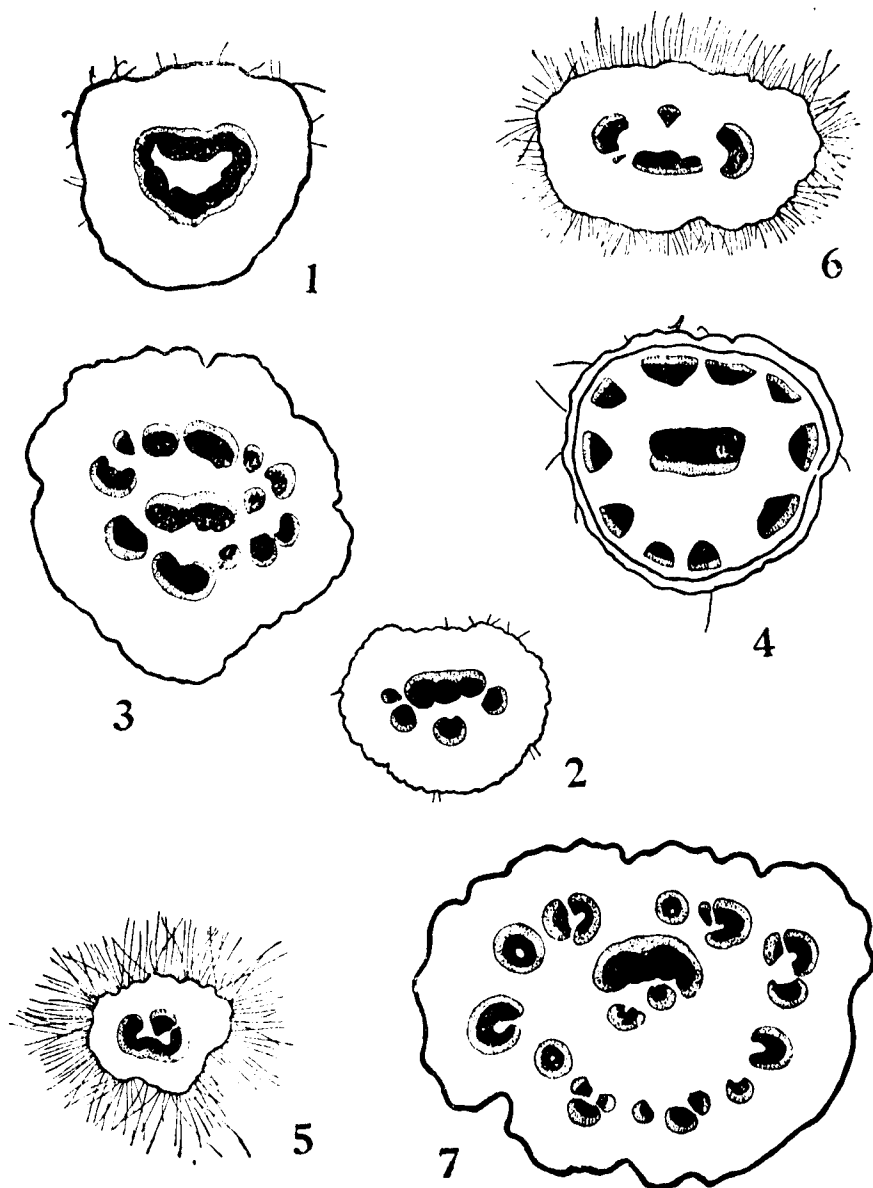
TEXT FIGURES 1-7. Transections of petioles.
