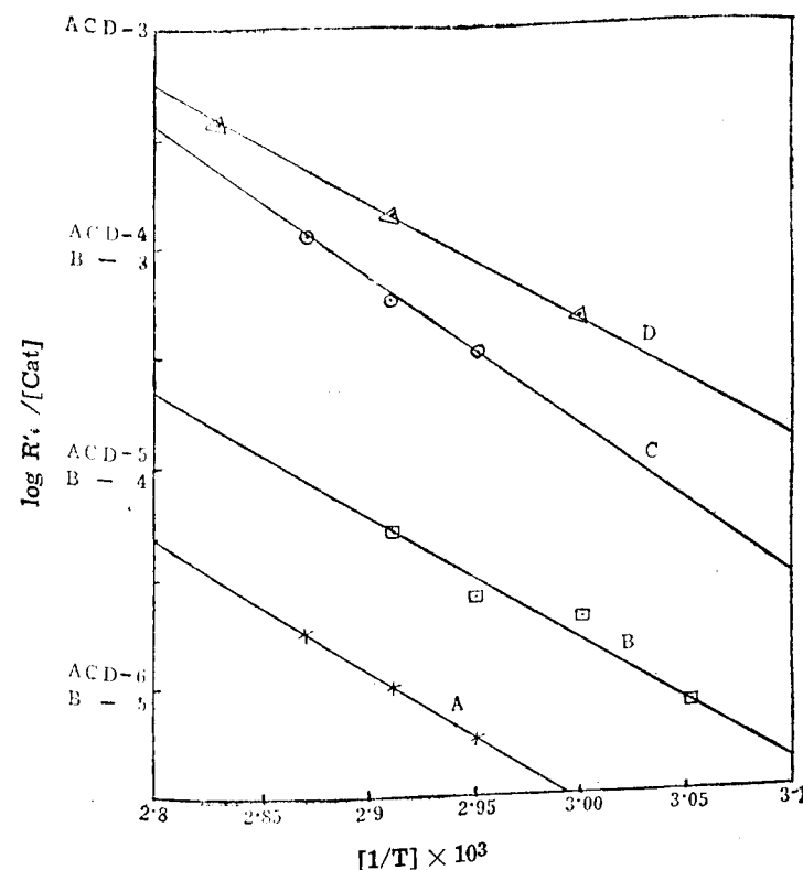
FIG. V. Plots A, B, C & D refer to the variation of R'_i/[Cat] with temperature when DTBP, Bz_2O_2 , MEKP and Azo respectively were used as initiators.
