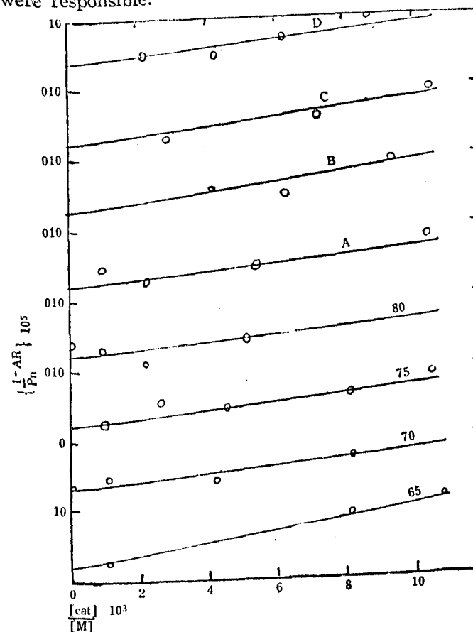
FIG. 4. \{(1/P_n) - AR\} vs. [Cat]/[M] in Bulk at temperatures 65°, 70°, 75° and 80°C and in solution A (Ethylacetate), B (Benzene), C (Toluene), D Methyl Ethyl Ketone at 70°C.
