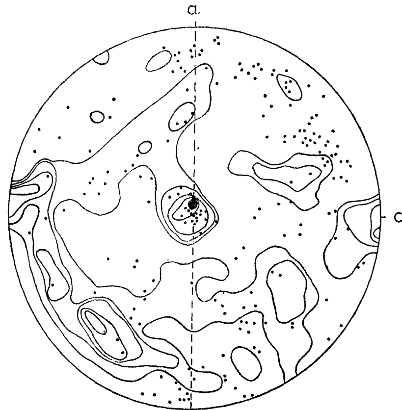
FIG. 17 Petrofabric diagram of 200 quartz grains. Contour interval 1% maximum 11%.
