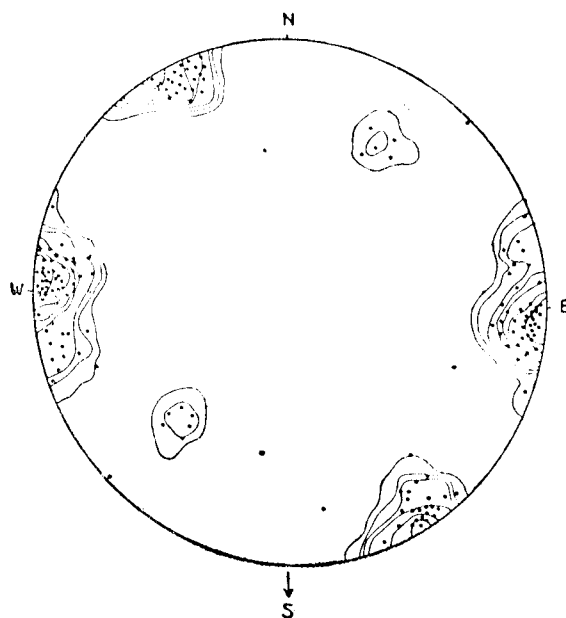
FIG. 15 Contours at 0-1-2-3-6-9-12-15% (163 Poles).
