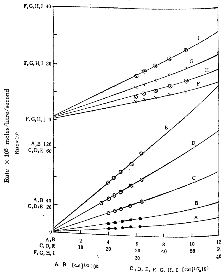
FIG. II. Plots A & B give the relationship between R_p and (\text{Cat})^{1/2} in the polymerization of methyl acrylate with \text{HAzo} as initiator at 70^\circ\text{C} and 80^\circ\text{C} respectively, with a 20 per cent solution of the monomer in ethyl acetate. Plots C, D & E give the same relationship with \text{Azo} as initiator at 60^\circ\text{C} , 70^\circ\text{C} and 80^\circ\text{C} respectively, with a 20 per cent solution of the monomer in ethyl acetate.
