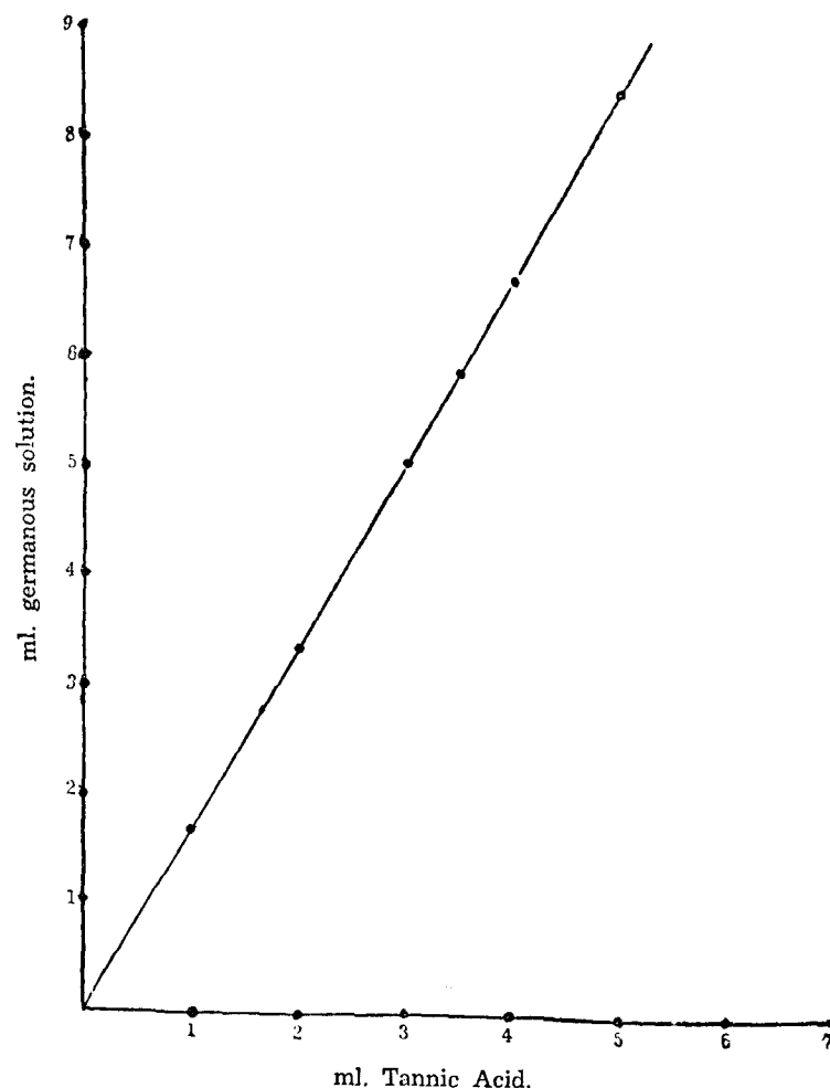
FIG. 3 Calibration Curve.
