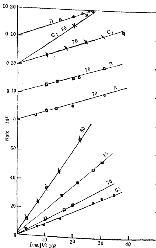
FIG. 2. Rate vs. (Cat)^{1/2} in Bulk at temperatures 65°, 70°, 75 and 80°C from below and in solution (4.6 molar).
