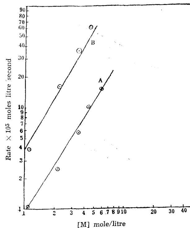
FIG. I. Plot A gives the relationship between \log R_p and \log M in the polymerization of methyl acrylate with Bz_2O_2 as initiator at 60^\circ C in ethyl acetate solution. The values are plotted on the Logarithmic Scale.
