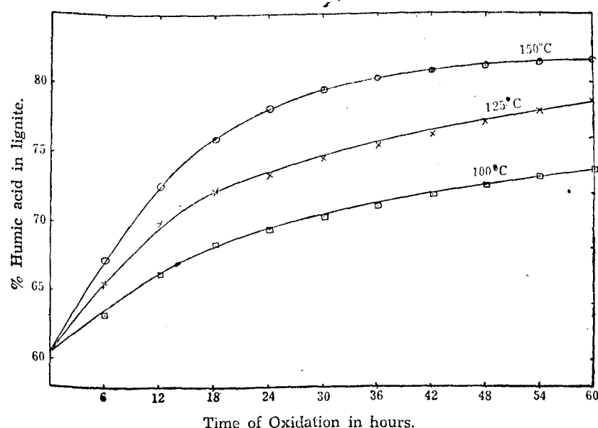
FIG. 3 Oxidation of Lignite in a fluidised bed (Method II)
