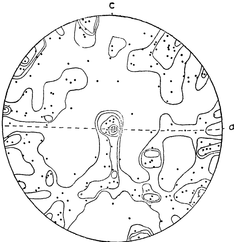
FIG. 16 Petrofabric diagram of 200 quartz grains. Contour interval 1% maximum 5%.
