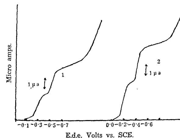
FIG. 1 Polarograms of + 2. Ge in 0.5N HCl and 1M. Ammonium Sulphate. 1. 8 \times 10^{-4} M Ge. 2. 1.2 \times 10^{-3} M Ge.
