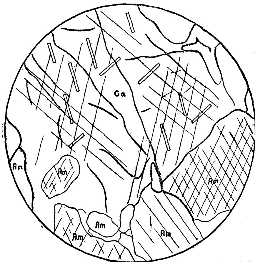
SKETCH 3: Garnet has developed hexoctahedral partings and inclusions arranged parallel to the cubic faces.
