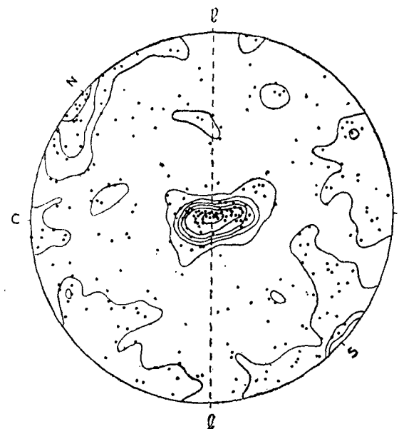
FIG. 20-c Contours at 0-1-2-3-4-5-7% (234 Quartz axes).
