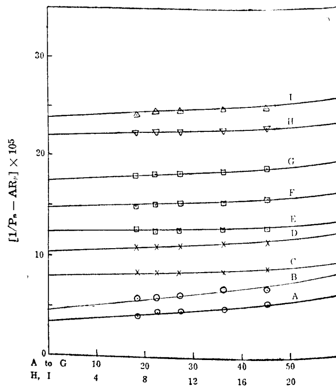
FIG. VI. All the Plots give the variation of [1/P_n - AR_p] with [Cat]/[M] in the polymerization of methyl acrylate with a 20 per cent solution in ethyl acetate.
