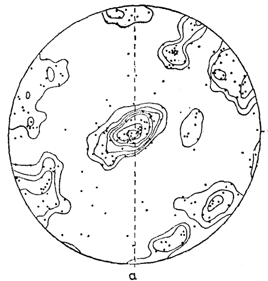
FIG. 20-b Contours at 0-1-2-3-4-5-6-7% (266 Quartz axes).
