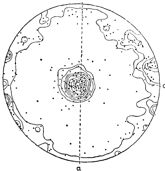
FIG. 20-a Contours at 0-1-2-3-4-5-7-9-11% (231 Quartz axes).
