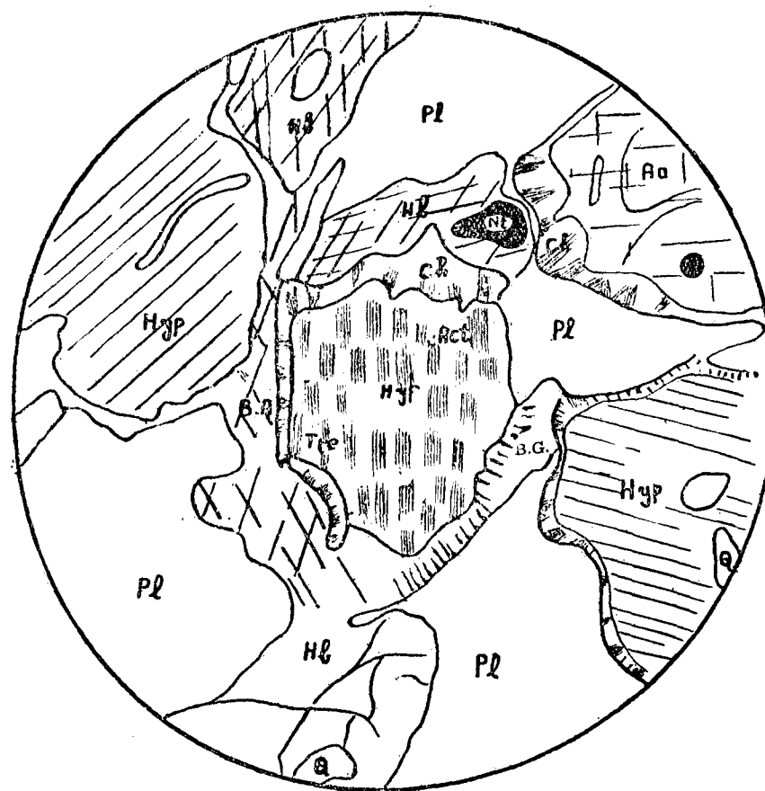
SKETCH 1: Hypersthene completely replaced by actinolite and tremolite. Augite and hypersthene grains are surrounded by a rim of chlorite and blue green hornblende. At contacts with hypersthene and plagioclase, brown amphibole develops.
