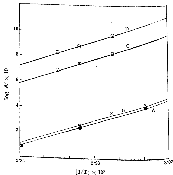
FIG. IV. Plot A log A' vs. 1/T with Azo. Plot B log A' vs. 1/T with Bz_2O_2 . Plot C log A' vs. 1/T with DTBP. Plot D log A' vs. 1/T with MEKP.
