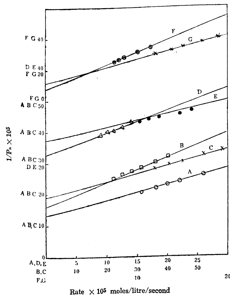
Fig. III. Plots A, B & C give the relationship 1/P_n vs. R_p with Azo as initiator at 60°C, 70°C and 80°C (2.2 molar monomer).
