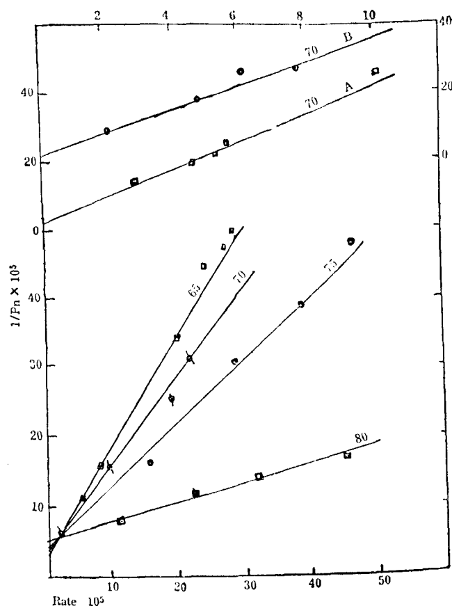
FIG. 3. Rate vs. 1/P_n in Bulk at 80°, 75°, 70 and 65°C from below and in solution. A Ethyl Acetate, B Benzene at 70°C.
