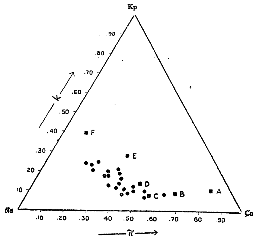
Fig. 5. k-\pi diagram of Lassen Peak (after Niggli)
