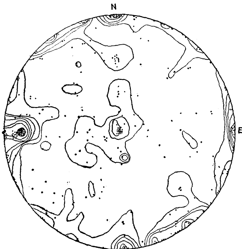
Fig. 1. Contour diagram of poles of Jt planes. 300 points. Contour interval 1%. Maximum 8%.
