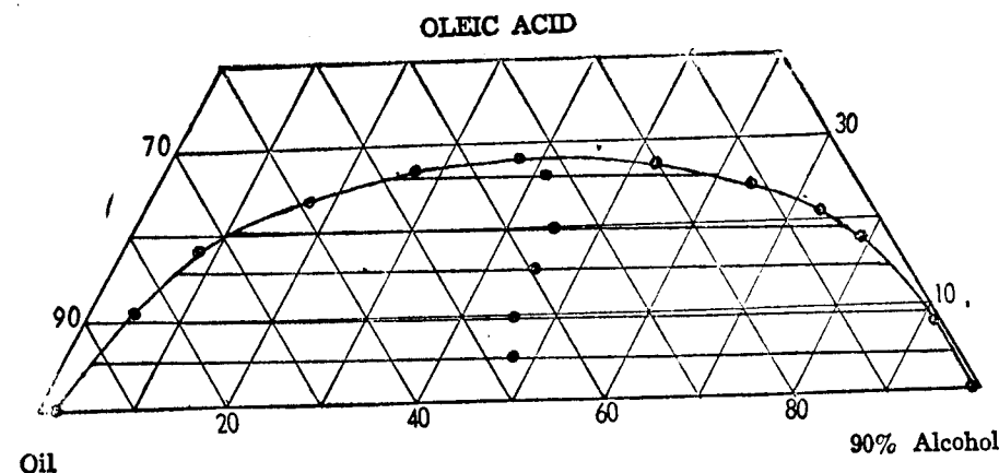
Fig. 3. Solubility curve and Tie lines for the system: Groundnut oil—Oleic acid—90% Alcohol.
