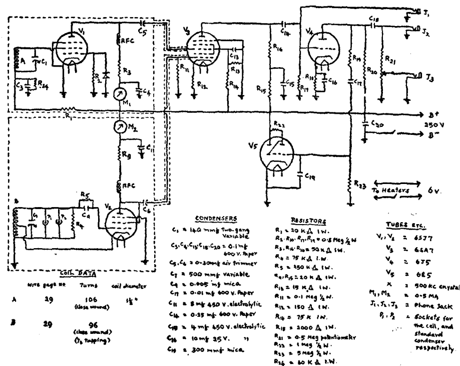
MODIFIED HETERODYNE BEAT APPARATUS OF JEN-YUAN CHIEN J. chem. edn. 24, 494 (1947)
