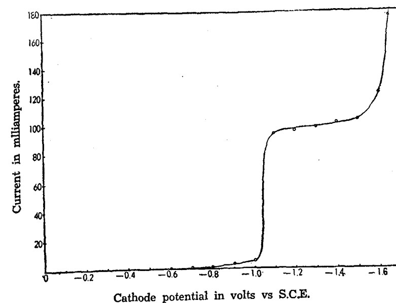
Fig. 2. Current-Cathode Potential Curve for Deposition of Tin from an alkaline solution containing 50 mg. of Tin in 200 c.c.
