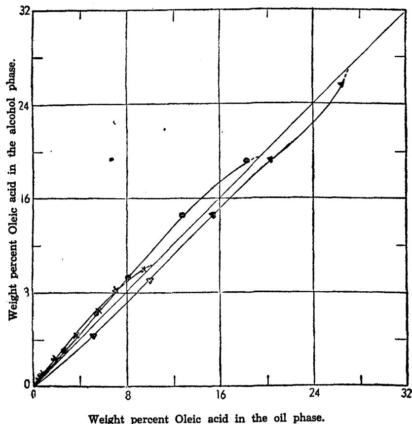
Fig. 4. Distribution of Oleic acid between the oil and the alcohol phases. × Anhydrous alcohol ○ 95% alcohol ▼ 90% alcohol
