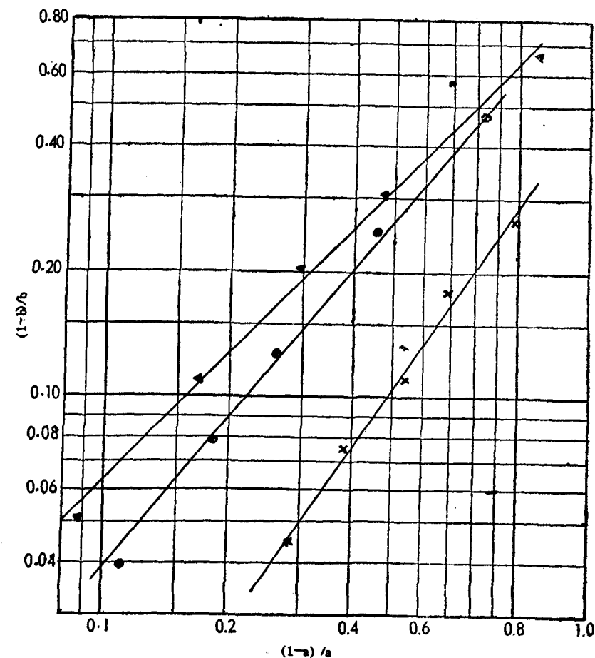
Fig. 5. Correlation of Tie line data.
