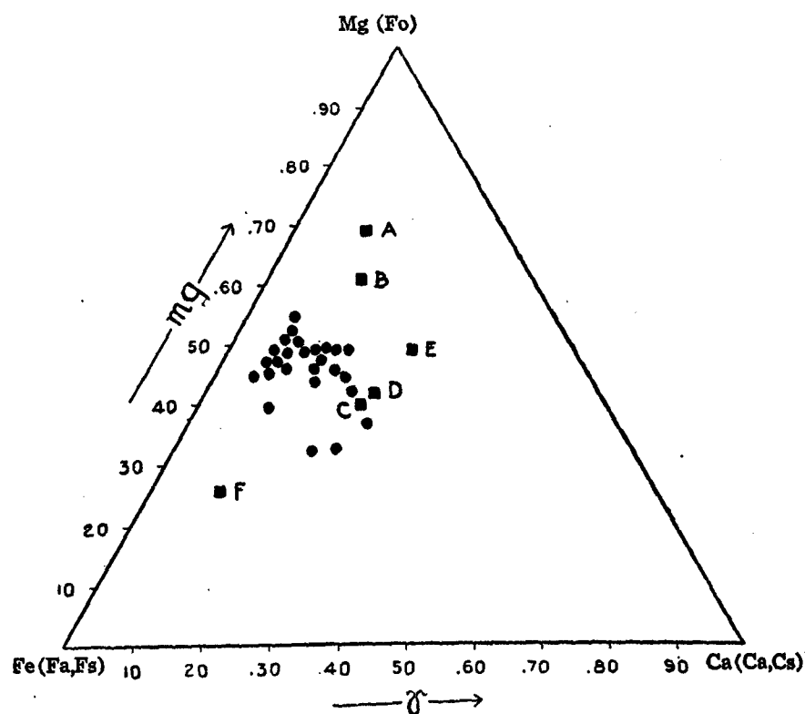
Fig. 6. mg- \gamma diagram of Lassen Peak (after Niggli). ■ = Dyke rocks of Pallavaram.
