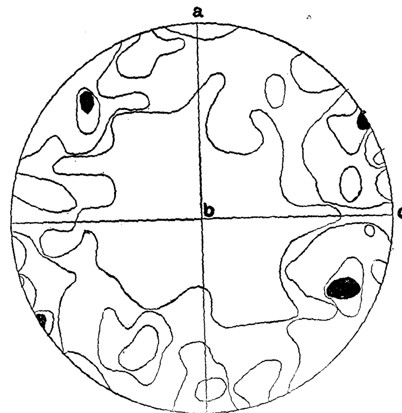
Fig. 2. Petrofabric diagram of Biotite gneiss. 300 quartz grains. Contour interval 1%. Maxima 4%.
