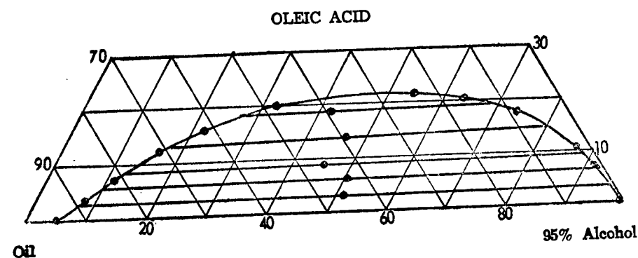
Fig. 2. Solubility curve and Tie lines for the system: Groundnut oil—Oleic acid—95% Alcohol.
