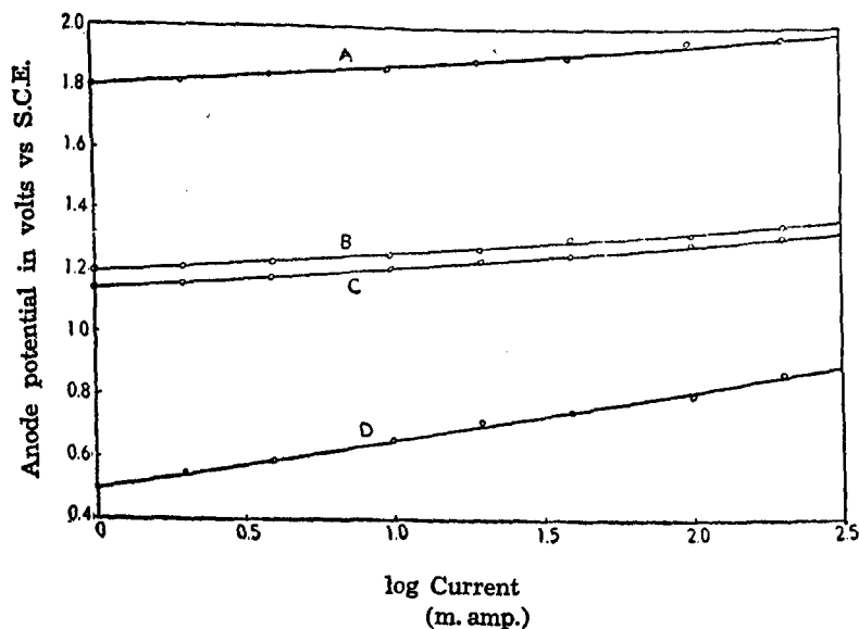
Fig. 1. Plot of Anode Potential vs Logarithm of current in a solution containing 200 mg. of Tin in 100 c.c.
