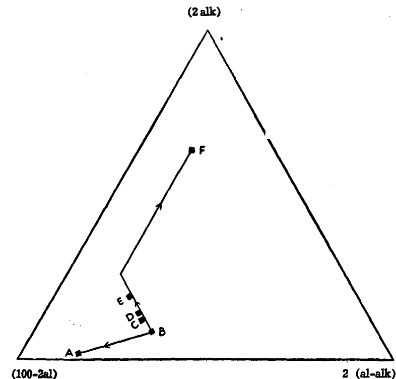
Fig. 7. Normative mineral diagram. ■ = Dyke rocks of Pallavaram.
