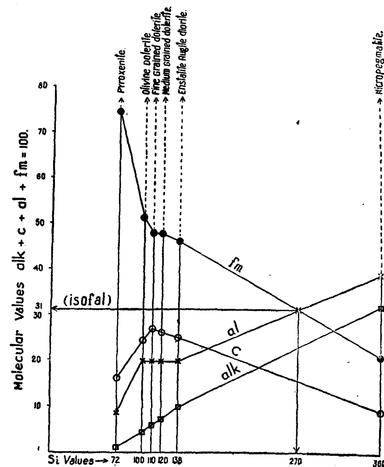
Fig. 3. Variation Diagram of the dyke rocks of Pallavaram. al = fm at 31, si = 270.
