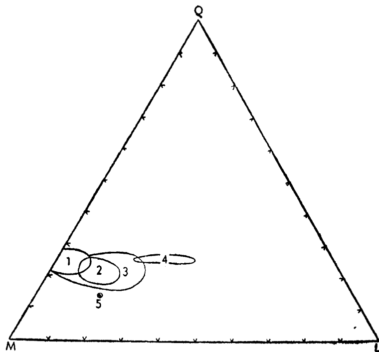
FIG. 1: Niggli's Q, L, M diagram for pyroxenes.
