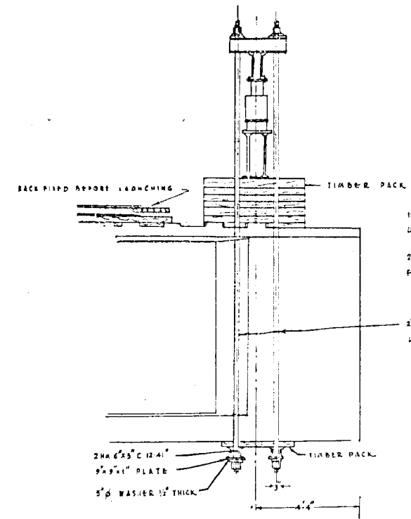
SIDE VIEW OF SUSPENDED BEAM.
