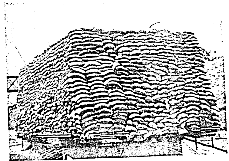
Photo 2. Kentledge for sinking well in stiff clay
