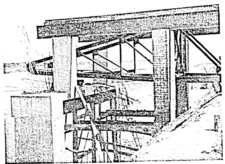
Photo 13. Steel launching girder moving to position
