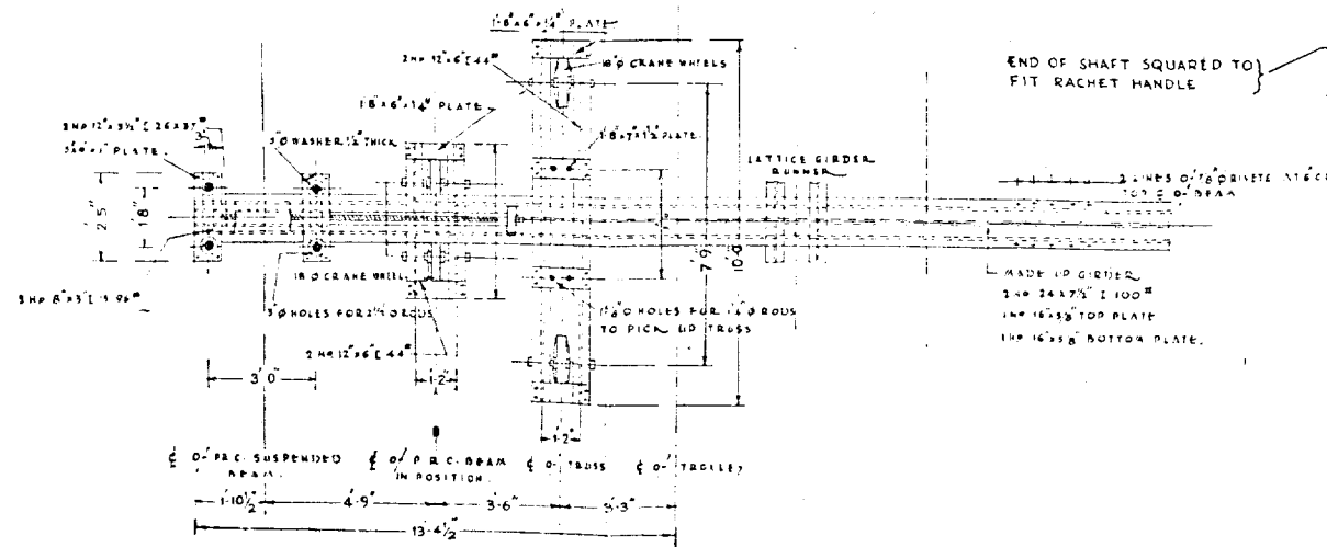
HALF SECTION SHOWING SUSPENDED BEAM IN TRANSIT.
