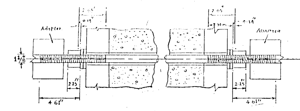
BEFORE STRESSING
