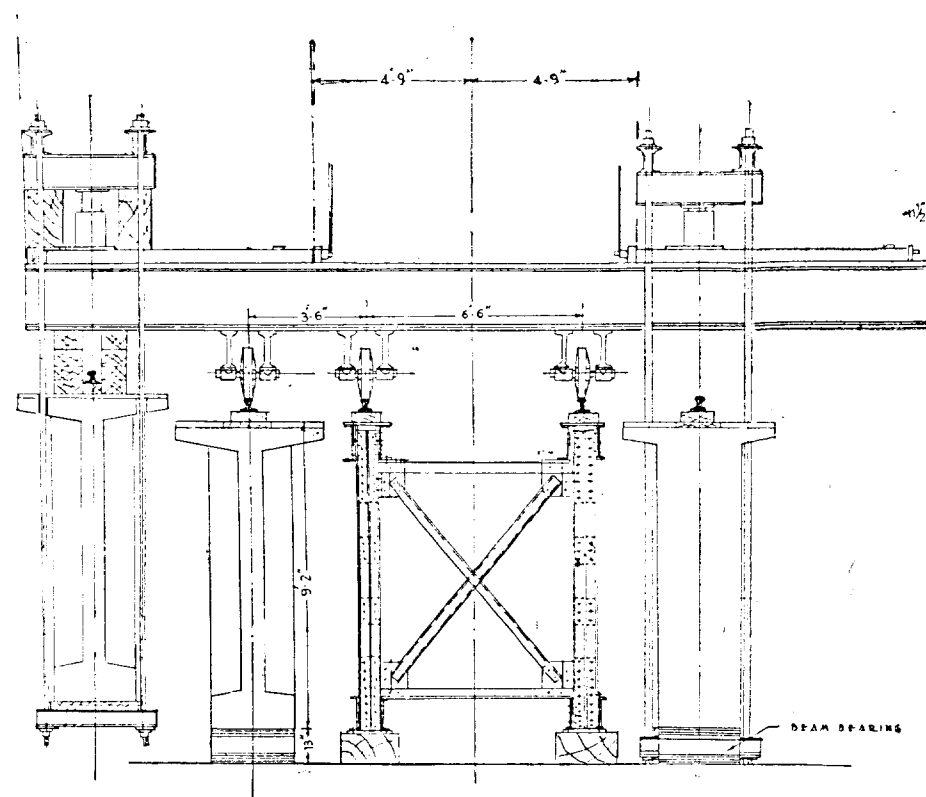
HALF SECTION SHOWING SUSPENDED BEAM IN TRANSIT.
