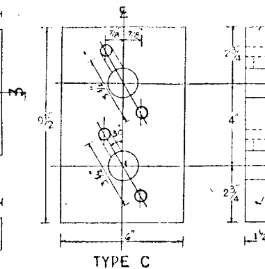
END PLATES FOR "MACALLOY" BARS
