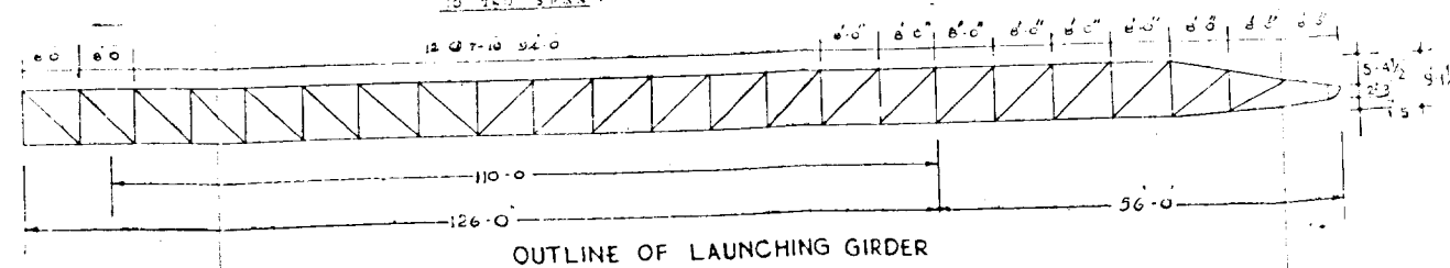
VARIOUS STAGES OF LAUNCHING GIRDERS MAHI BRIDGE
