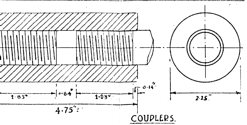
FORM OF LEE McCALL HIGH EFFICIENCY NUTS & COUPLERS.
