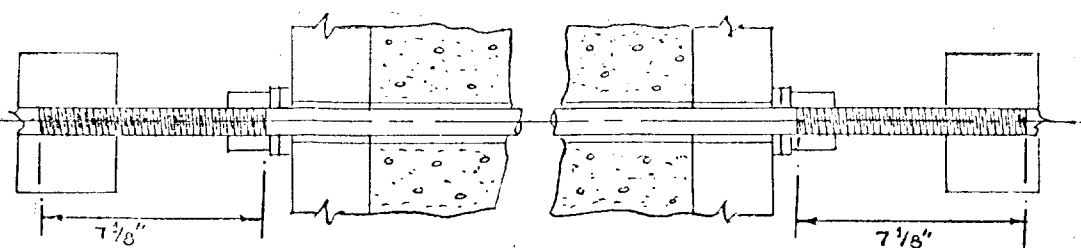
AFTER STRESSING
