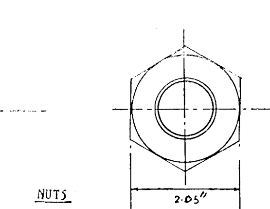
FORM OF LEE McCALL HIGH EFFICIENCY NUTS & COUPLERS.
