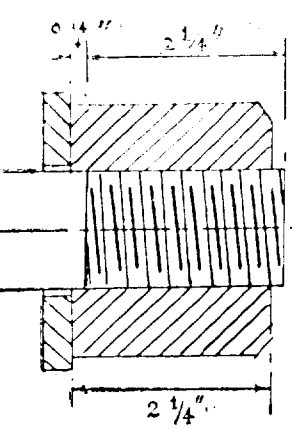
FORM OF LEE McCALL HIGH EFFICIENCY NUTS & COUPLERS.
