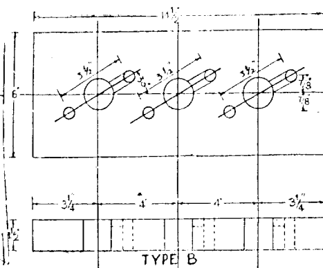
END PLATES FOR "MACALLOY" BARS
