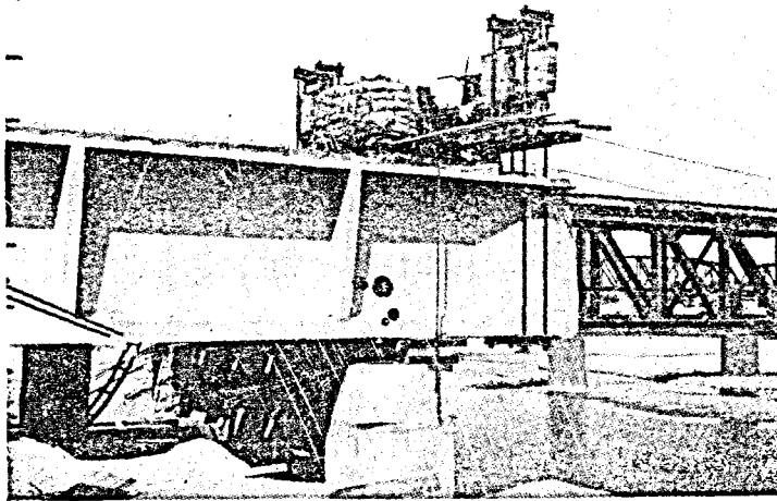
Photo 15. Precast prestressed girders being launched
