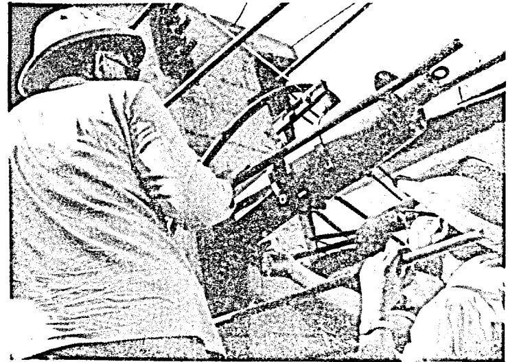
Photo 9. Prestressing operation—reading the vernier
