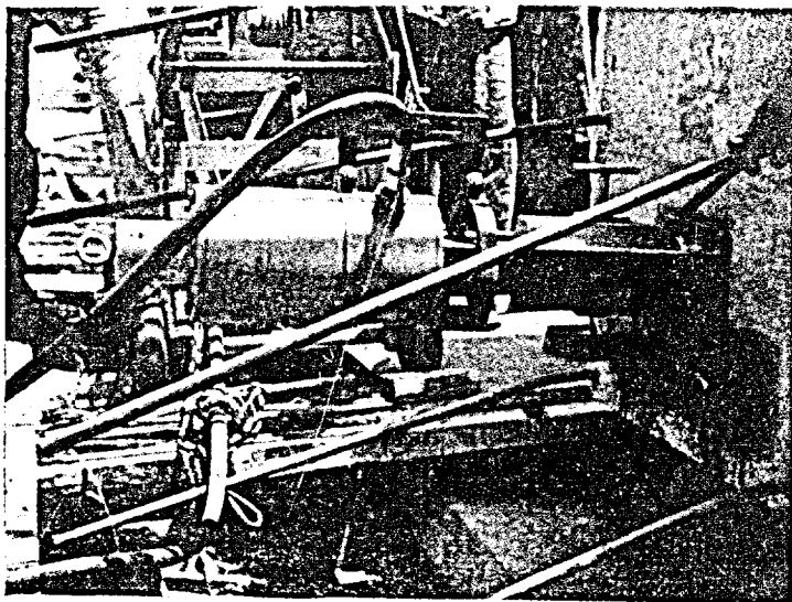
Photo 8. Prestressing jack
