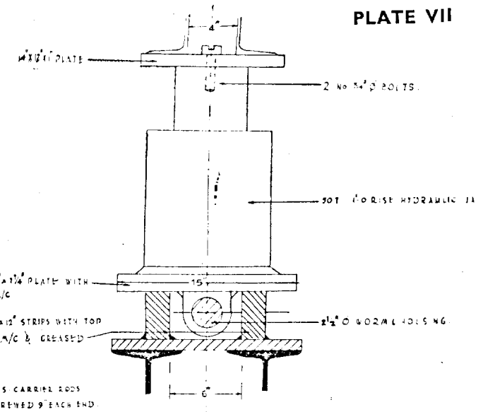
DETAIL OF JACK & TRAVERSE FIXING.
