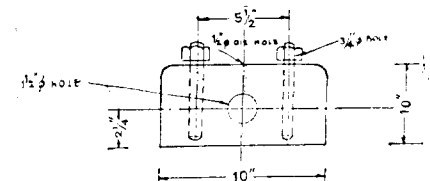
DETAIL OF THRUST BLOCK.
