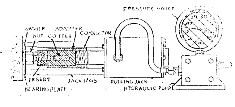
LEE-McCALL 42 TONS SPECIAL JACK.
