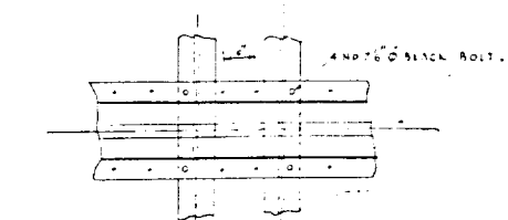
DETAIL OF JOINT BETWEEN GIRDER & RUNNER.
