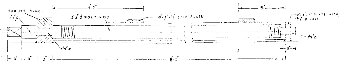
DETAIL OF TRAVERSING DEVICE.
