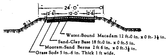
Fig. 3. Cross section in sandy sub-grade
