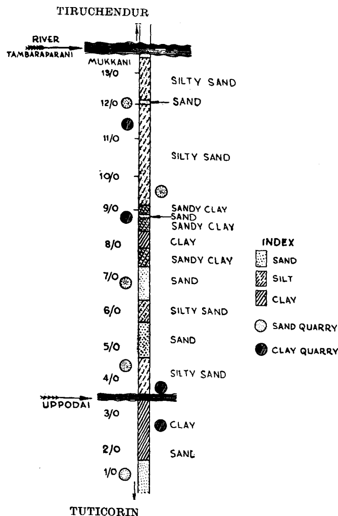
Fig. 2. Types of subgrade soils and location of quarries
