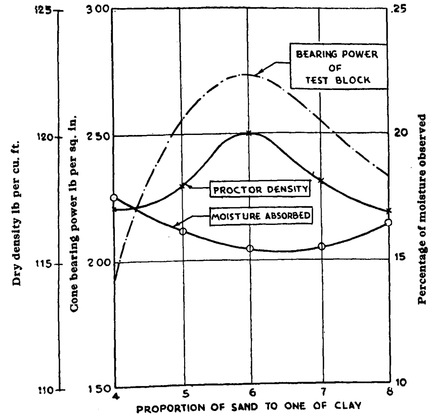
Fig. 6. Test results for design of mix for base course
