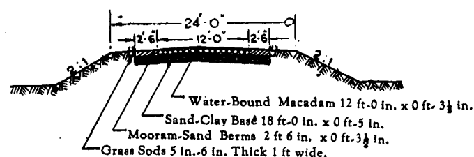
Fig. 3. Cross section in sandy sub-grade
