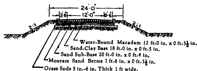
Fig. 4. Cross section in clay sub-grade
