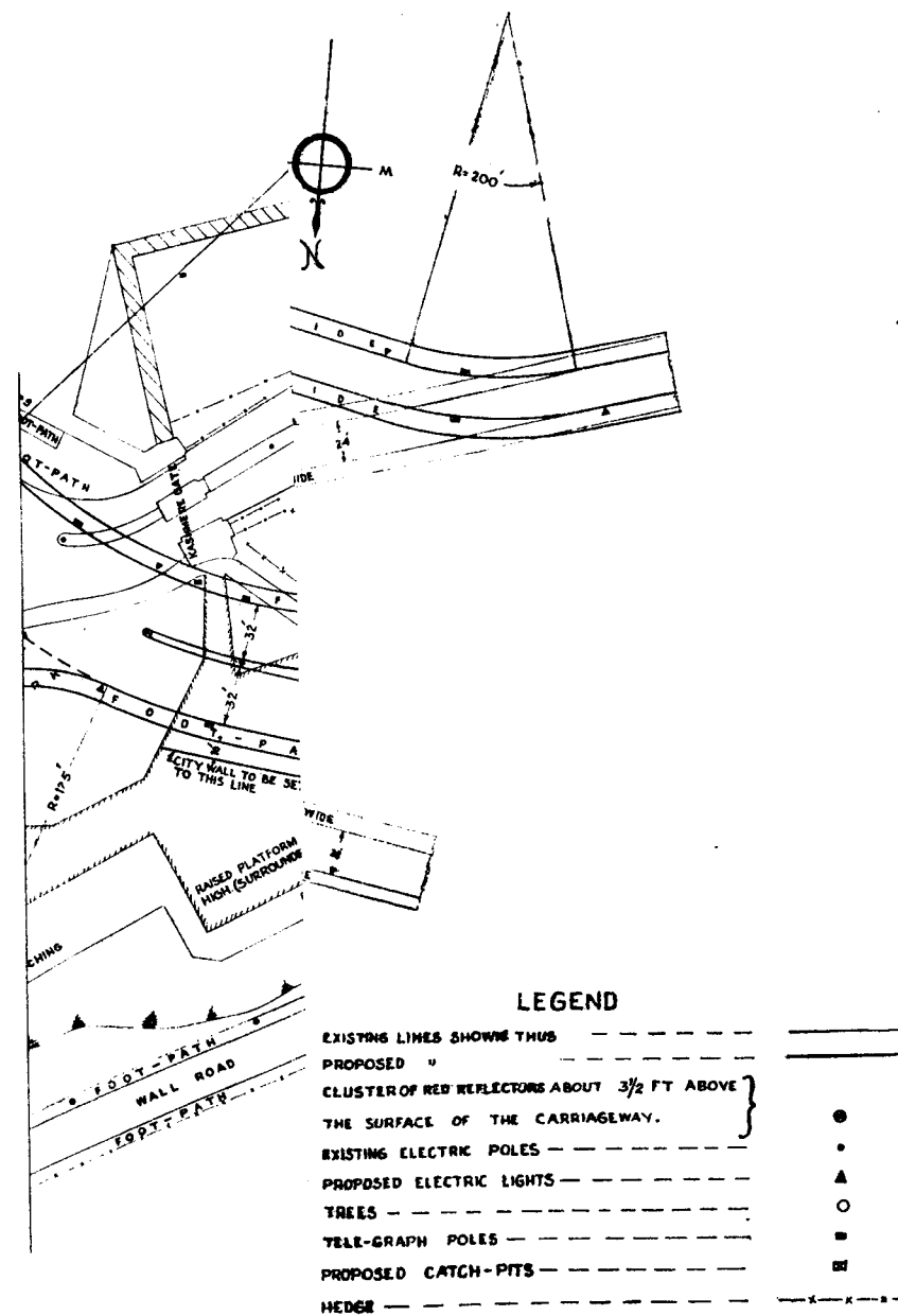
IMPROVEMENTS TO THE KASHMERE GATE JUNCTION, DELHI
