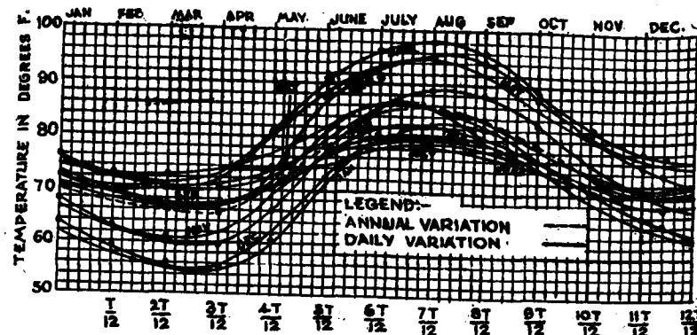
Fig. 10. Variation of diurnal and annual temperature at Poona,
