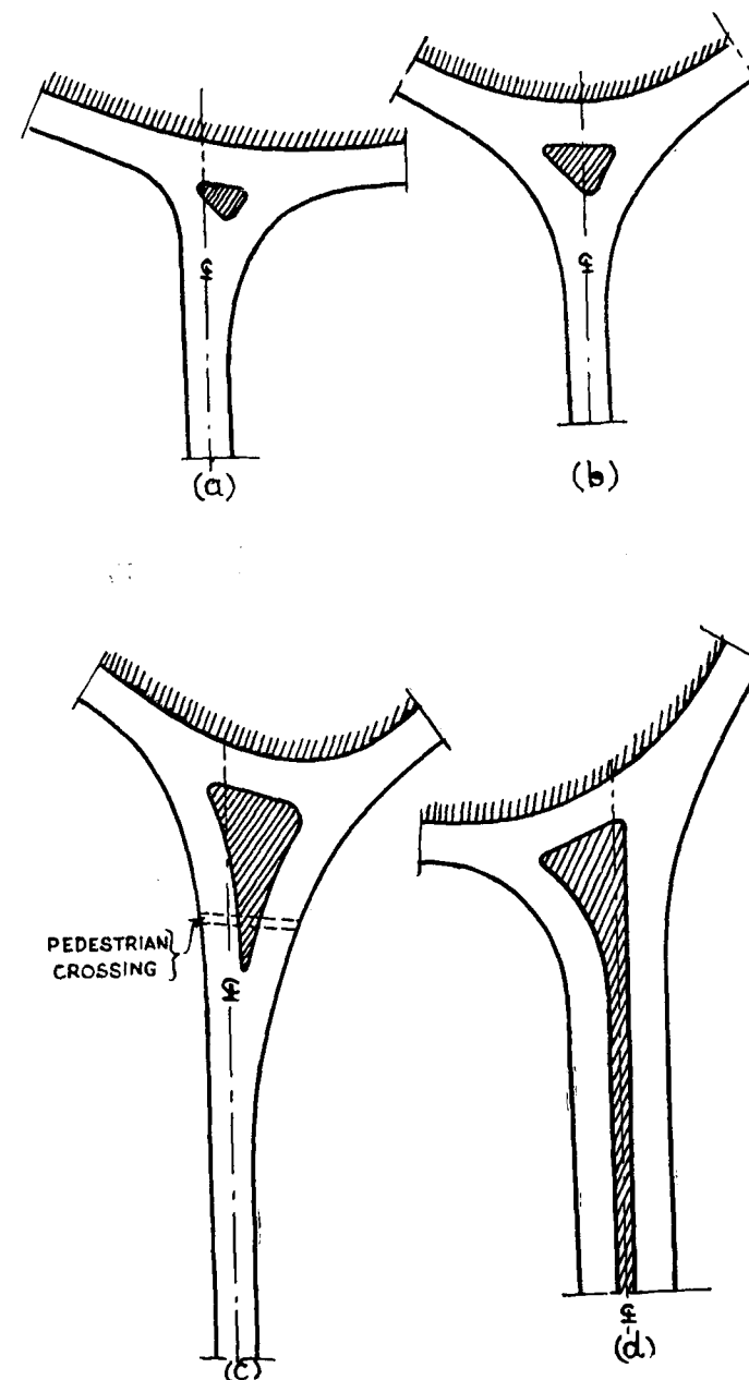
Fig. 13. Channelling island
