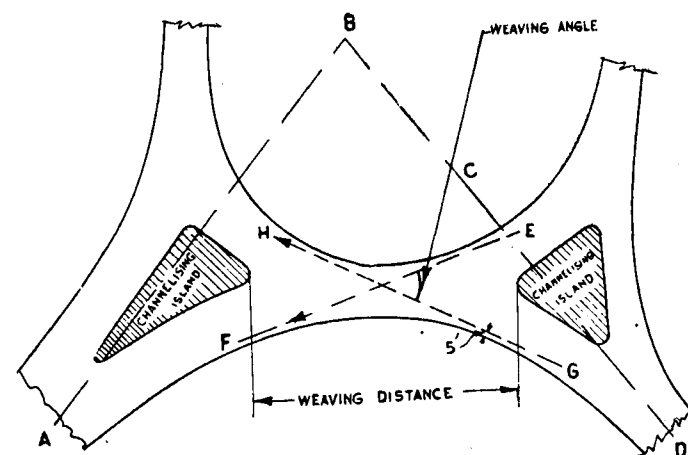
Fig. 4. Weaving angle & weaving distance
