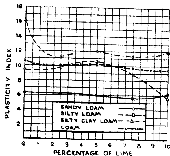
Fig. 1. Effect of Lime on the Plasticity Index
