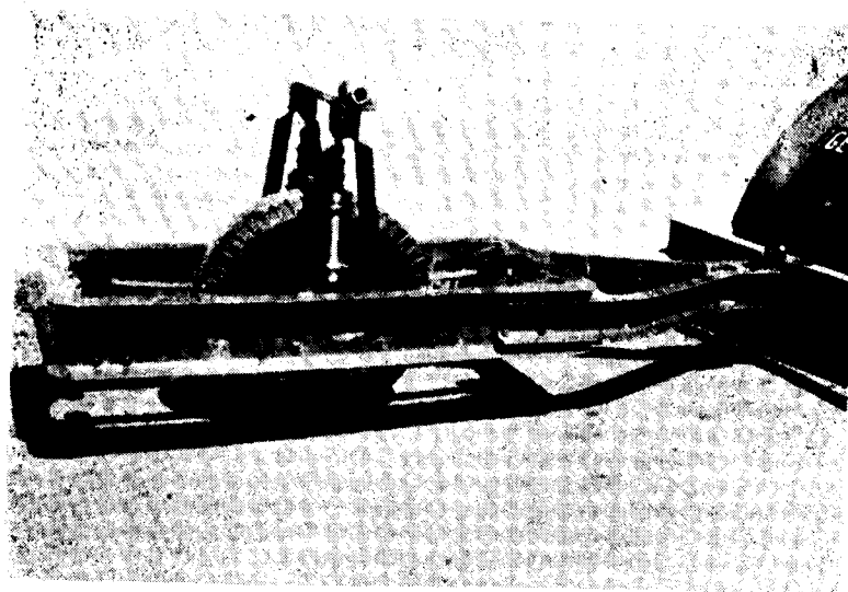
Photo 9. Roughometer
