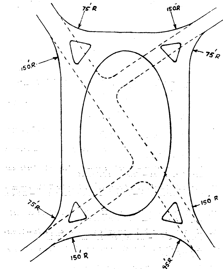
Fig. 20. Conversion of a Staggered intersection to a Rotary Junction
