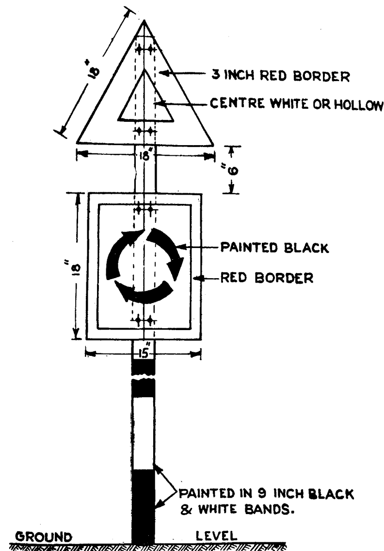
Fig. 17. Cautionary sign—rotary
