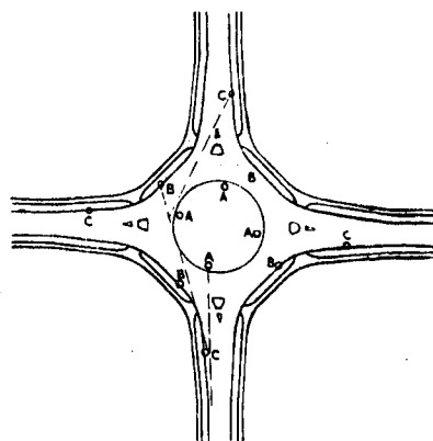
Diagram showing the standard way of lighting on intersection with a central island
