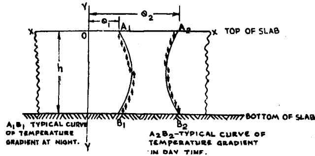
Fig. 9. Temperature gradient
