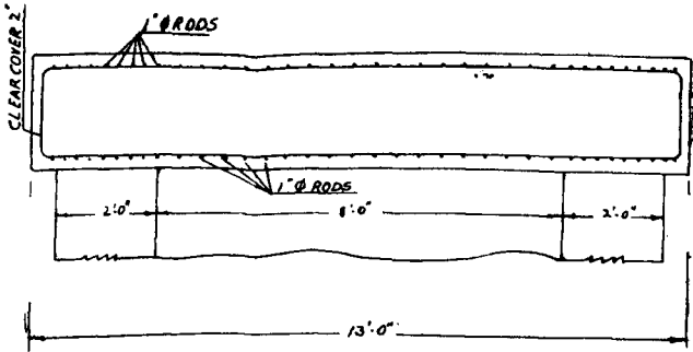
SECTION ON BB SCHEDULE OF REINFORCEMENT
