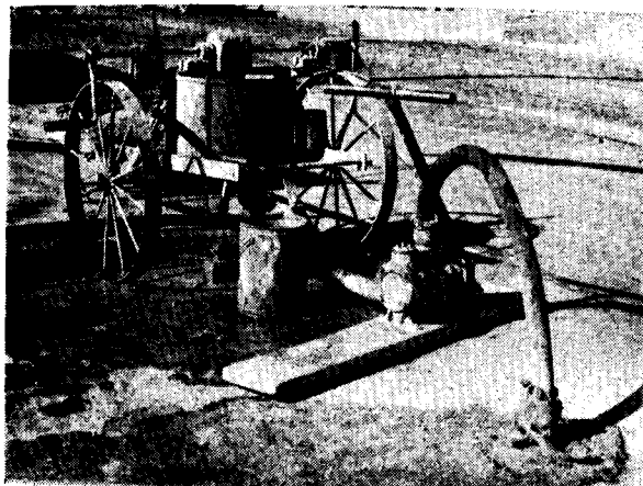
Photo 5. Raising concrete pavement by mud-jacking process. General view of machine
