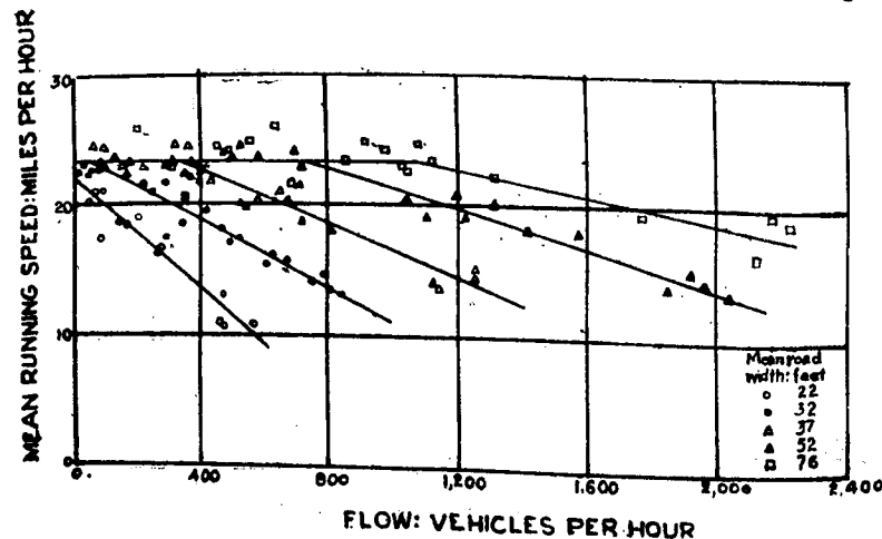
Fig. 18. Relation between mean running speeds and total flow in central London
