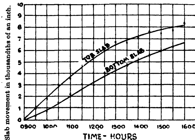
Fig. 13. Movement of concrete slabs when a separating layer of bitumen 80/100 and sand is applied at 8 lb per 5 sq. ft.
