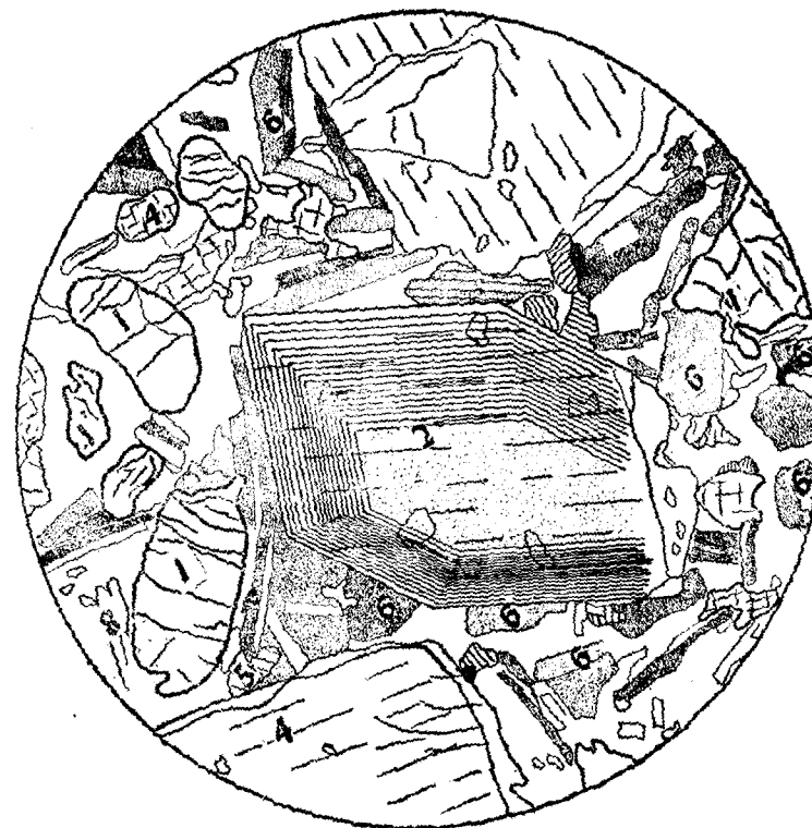
FIG. 1. Showing Zonary banding in augite. The bands, sometimes as many as thirty-five in number, show slight variation of extinction angles. The augite is poikilitic with olivine. The different shades of mottling in orthoclase indicates twinning after carlsbad law.
