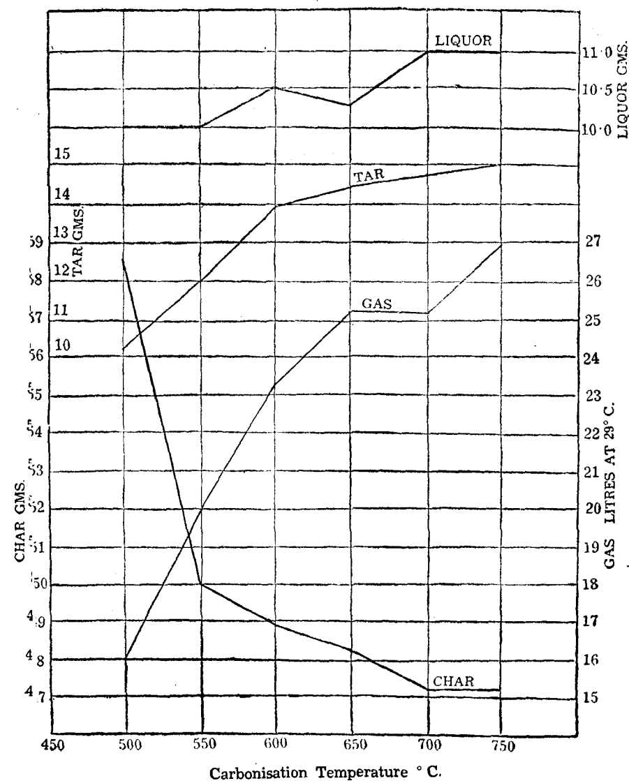
FIG. 1. Yield of Products on Carbonisation of 100 gms. of Moisture-Free Lignite.
