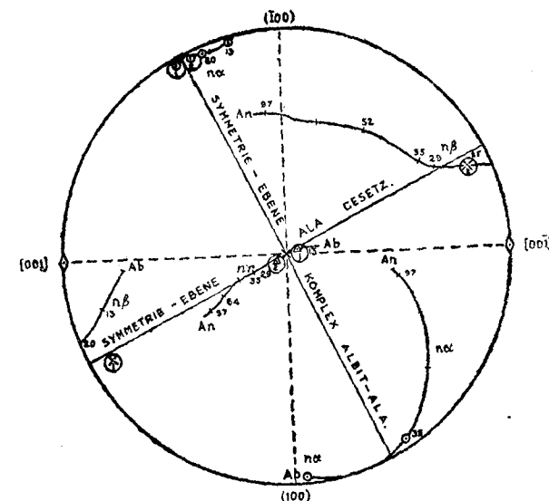
FIG. 4. Position of the transferred ellipsoidal axes for Albite-ala according to Plate 3 of Reinhard for An % 25.
