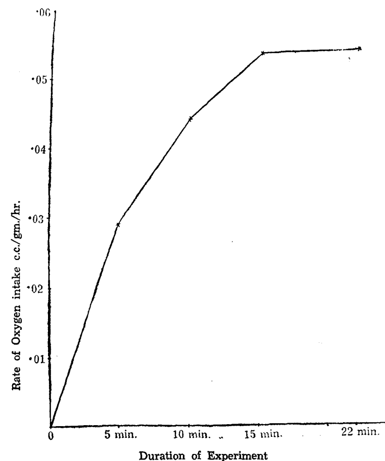
TEXT FIG. 2. Oxygen intake through skin when the frog is denied access to air.
