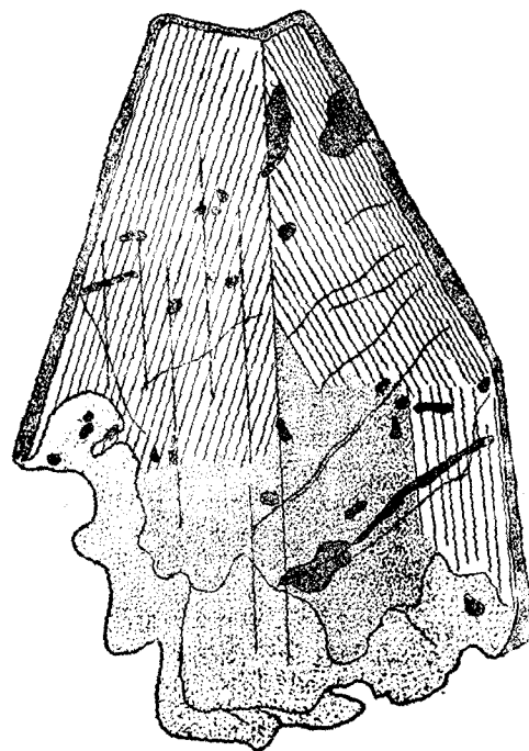
FIG. II. Herring bone structure in twin of augite, twinned after (100). The bands are parallel to the prismatic faces of the two individuals.
