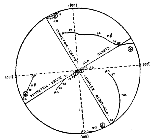
FIG. 5. Position of the transferred ellipsoidal axes for Albite law according to Table 3 of Reinhard for An % 16.
