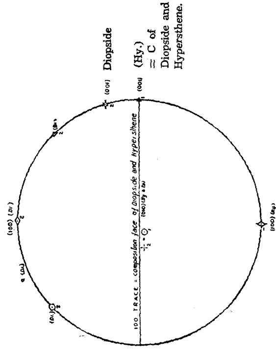
Fig. 6. Stereogram of parallel growth of Hypersthene and Diopside.
