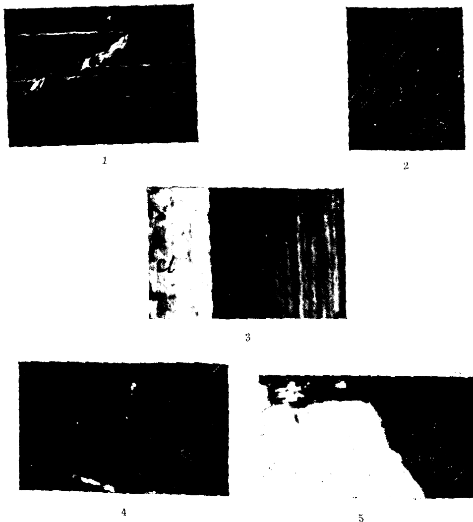
Figure 1. Lamellae parallel to (100) in orthopyroxene. The optic axial plane is parallel to the lamellae. The second individual appears as mere streaks of light. \times 120 ( \times Nicols).
