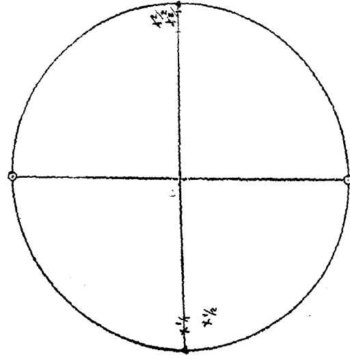
Fig. 7. Stereogram showing the positions of the twin-poles of the so-called herring-bone twins of Hypersthene.
