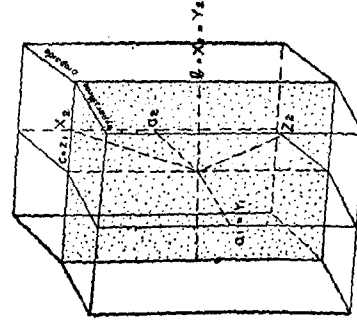
Fig. 5. Parallel growth of Hypersthene and diopside. dotted plane \equiv (100) of both
