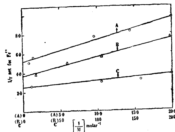
FIG. 3. Shows variation of 1/\gamma_{\text{net}} with reciprocal monomer concentration with \text{Fe}^{3+}\text{N}_3^- at \text{pH}=0.5 to 0.6 for acrylonitrile (Curve A), methyl methacrylate (Curve B) and methacrylic acid (Curve C).
