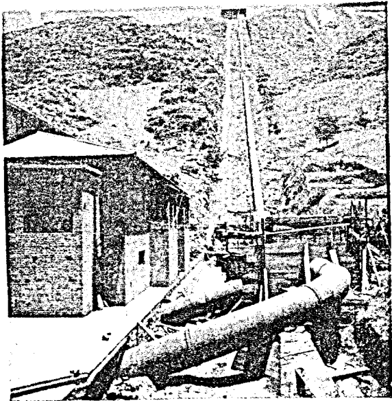
Photo 4. Penstock
