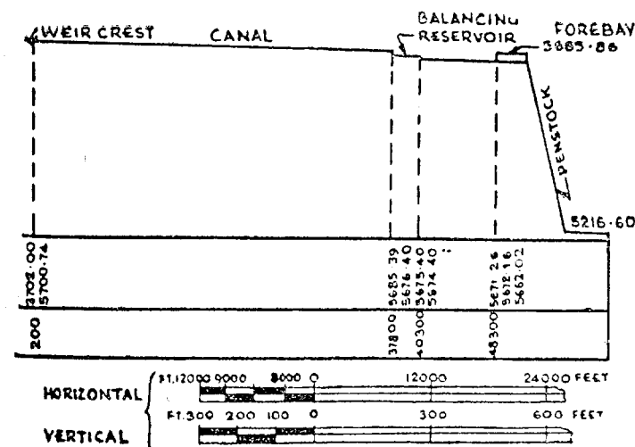
— L. SECTION OF CANAL —
