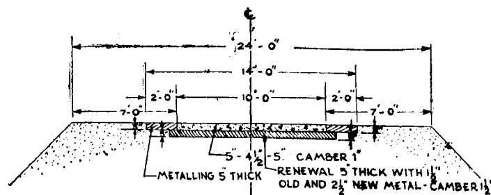
Fig. 3. Typical Section—Experiment in 97/5 to 98/8.
