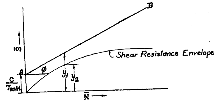
Fig. 2. \bar{S}-\bar{N} Curve and determination of Factor of Safety.
