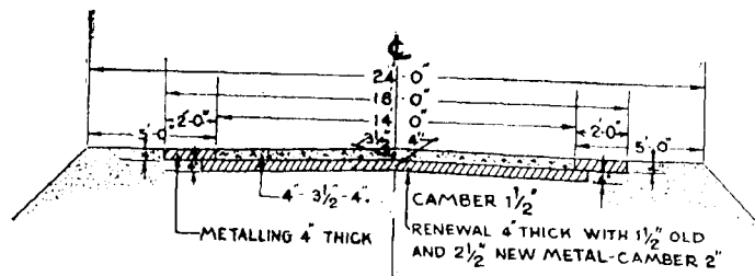
Fig. 1. Typical Section—Experiment in 93/4 to 94/3.
