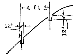
Furrow Section for Slope Planting
