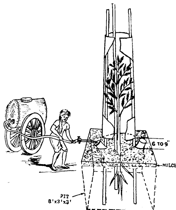
Fig. 14. The pot System of Irrigation
