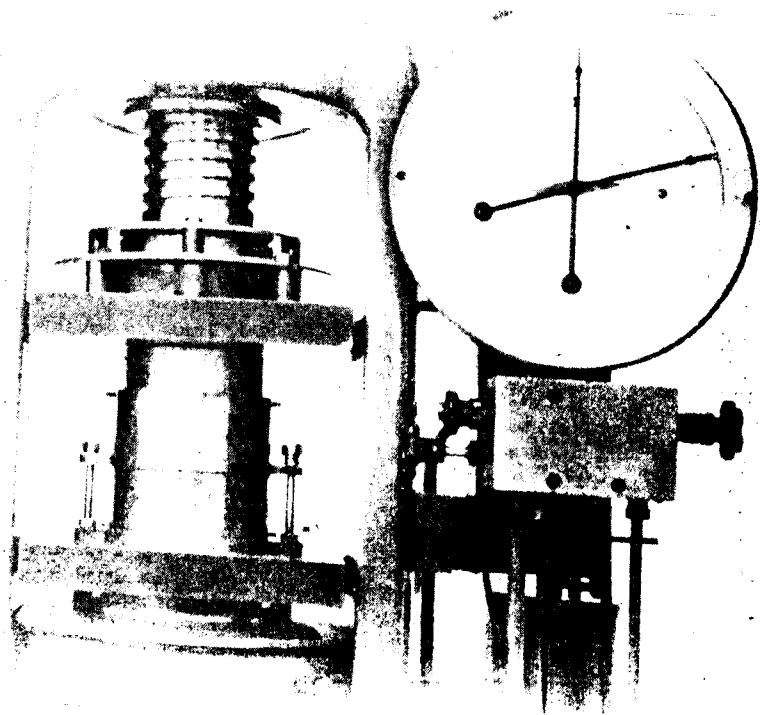
Photo 9. Arrangement for determining crushing value.
