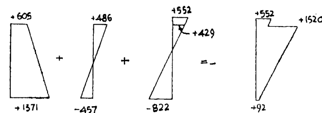
FINAL STRESS DIAGRAM FIBRE STRESSES.
