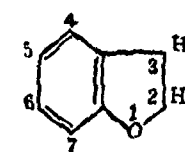
2, 3-dihydrobenzofuran
