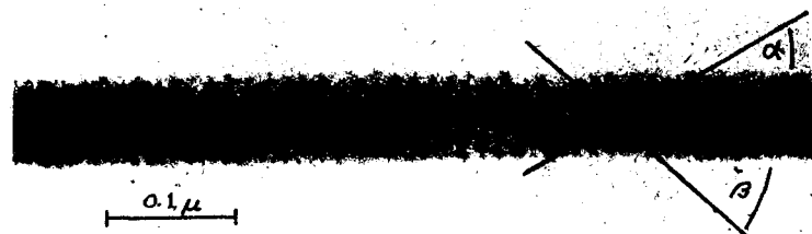
Plate 5. Electron micrograph of fibril from molluscan muscle, showing discrete spots which lie on diagonals which make different angles ( \alpha and \beta ) with the axis. (Courtesy of the Journal of Applied Physics ).
