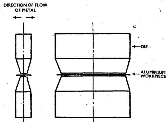
Fig. 6. – A pair of dies for pressing two pieces of aluminium into one continuous piece; end view on left, side view on right.
