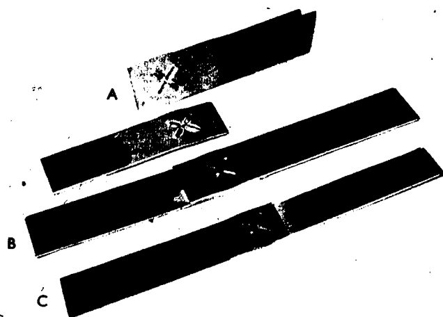
Plate 16. Strip-joints of aluminium (B) and aluminium to copper (C). (A) shows a typical tensile failure.
