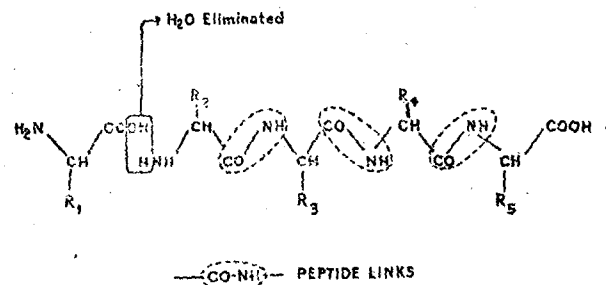
Fig. 8. — Polypeptide chain.
