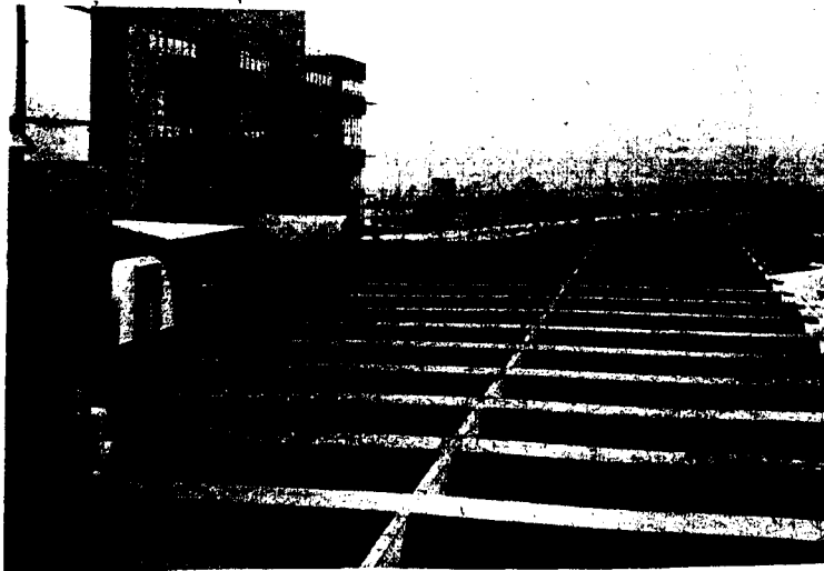
Plate 24. A view of the roof of a modern factory to show the system of north lighting. The huts on the roof house the intake fans for the ventilation system. The output is through the shafts rising up the sides of the multi-storey section on the left.
