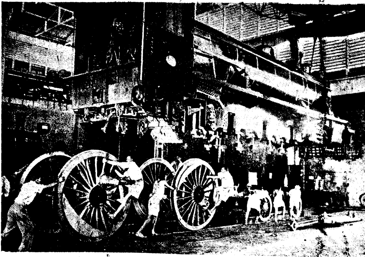
A steam locomotive being repaired in an Indian railway workshop. The wheels have been turned and the axle boxes relined with bearing metal and they are now being moved into position to receive the locomotive frame when lowered by the crane
