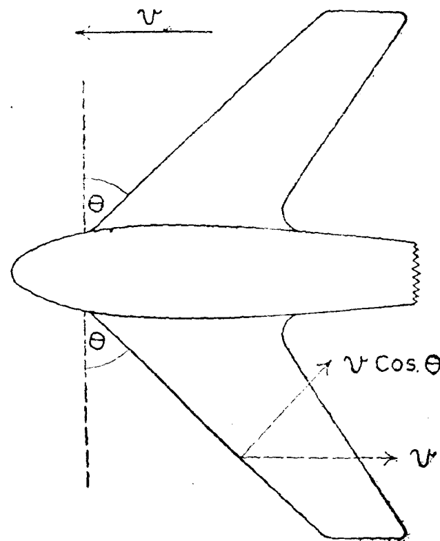
Figure 2—Aircraft with sweptback wings. v = velocity of the aircraft forwards, or of the air flow over it in the opposite direction. v \cos \theta = velocity of air flow perpendicular to the leading edge of the wings.
