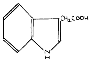
Indoleacetic acid.
