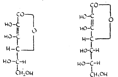
Glucoascorbic acid.
