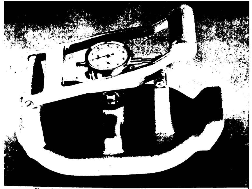
Plate 41. A hardness tester in which the penetration of a ball into the surface of the cheese under a standard load is measured. This serves as a kind of mechanical thumb and agrees fairly well with the grader's opinion. Kestra in Holland has made a similar study of the firmness of butter as judged by thumbing. Courtesy of Kraft Cheese Co.
