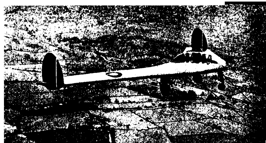
Plate 44. The Flying Wing. The quest for the flying wing, an aircraft without fuselage or tail-plane, has at last succeeded. The Armstrong Whitworth tailless glider was constructed to provide data for a larger power-driven flying wing (see Plate 46). It is believed that this highly efficient aerodynamic form, for which a great future is envisaged, will lead to the simplified structure of aircraft of great strength. The glider, which carries a pilot and engineer-observer, has a wing span of 54 feet, wing area 443 square feet and total weight of 6,000 lb. Photograph by Charles E. Brown.
