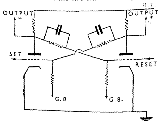
Figure 17—A flip-flop electronic counter circuit.
