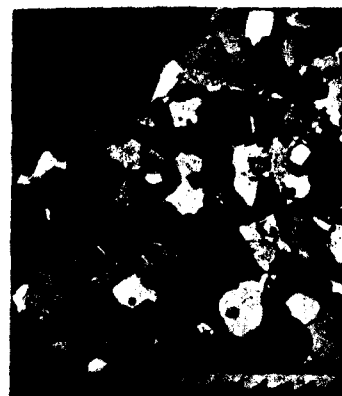
8 & 9 (a) Thin section of snow several years old, photographed between crossed nicols. This makes the crystals show up in bright colours. The blank regions are air spaces. (b) Thin section of glacier ice immediately below the firn line. The scale on both photographs is given by the teeth of the saw blade at the bottom which are 0.9 mm. apart.
