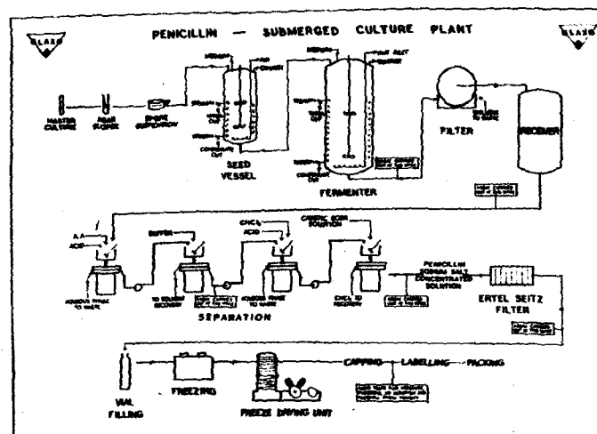
22. Flow sheet for Penicillin production.
