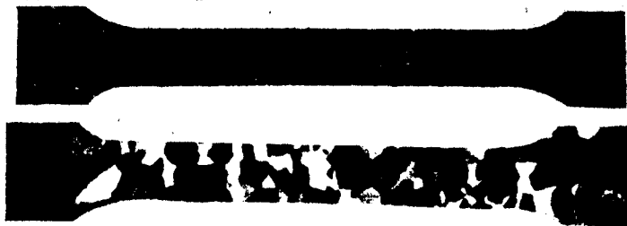
10. Etched strips of aluminium before extension and annealing (top) and after (bottom), showing crystal growth.
