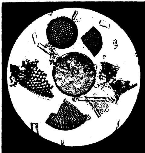
40. Diatoms recovered from one of the filtering elements of a "Metafilter."
