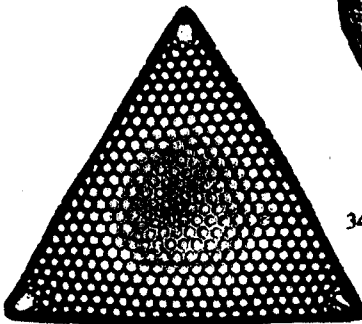
33. Lepidodiscus imperialis . Fossil species of exquisite design.
