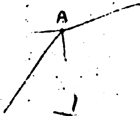
31. Atoms of the radioactive element thorium have been incorporated in the emulsion of a photographic plate. At A one of them has burst, giving off four alpha particles (helium nuclei) which have marked the emulsion in their passage. Two of the tracks look fuzzy because they are out of focus in this micro-photo of the plate. See page 57.
