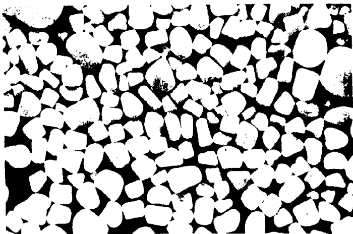
30. Concretions formed in underground water.
