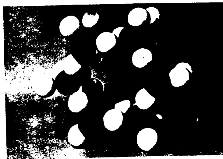
Plates 19-25 illustrate Rain (p. 104).
