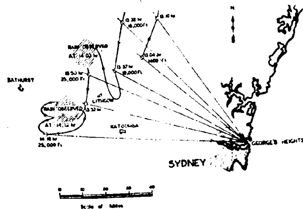
Figure 6—Radar plot of the aircraft track and the two areas where rain echoes were observed to form
