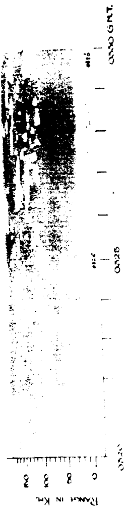
18. Ionisation trails associated with the Giacobini-Zinner Meteor shower on 10.10.46 and recorded at Radio Research Station, Slough. See Meteors and Radar p. 36.
