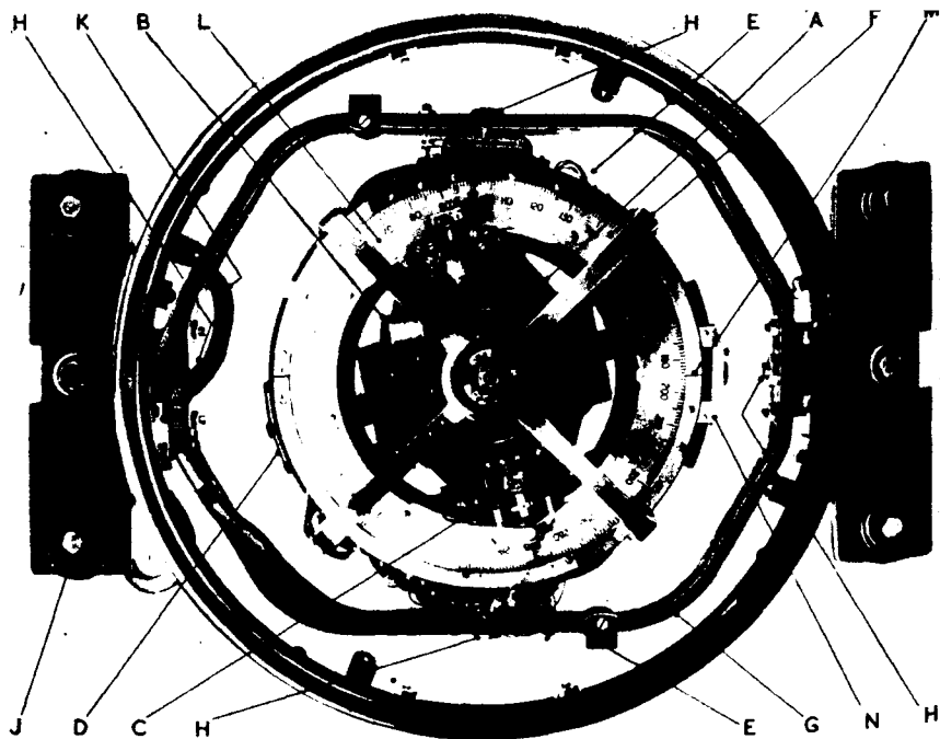
12. The master gyro-compass of the type used in the Royal Navy seen from above. This master transmits the direction of the ship's head to repeaters wherever they may be required in the ship. A, case containing the rotor which provides the directive force; B, gauge to indicate the vacuum in the rotor case; C, the contactor which passes a signal when the phantom is out of line with the rotor case; D, the Azimuth motor which drives the phantom after the rotor case; E, transmitters which are driven by the phantom and which send out impulses to the repeaters; F, the Spider which supports the moving parts; G, gimbal ring to maintain the compass with its card horizontal; H, gimbal pivots; J, shock absorbers to support the compass and protect it from the vibration of the ship; K, cable carrying electrical supply to and from the master; L, card; M, lubber line; N, corrector mechanism for making adjustments for speed and latitude.
