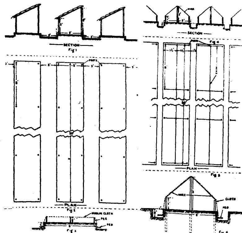
Plan and section of Virginia tobacco nurseries.
