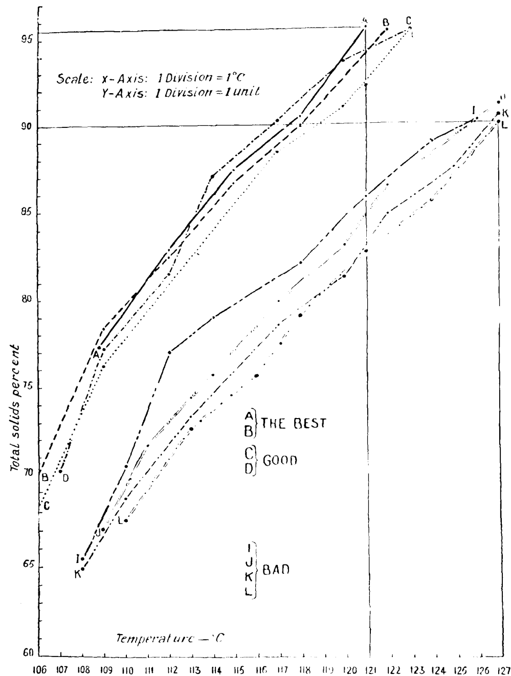
Graph showing the changes in concentration & the corresponding temperatures during the boiling down of the cane juice to Jaggery.
