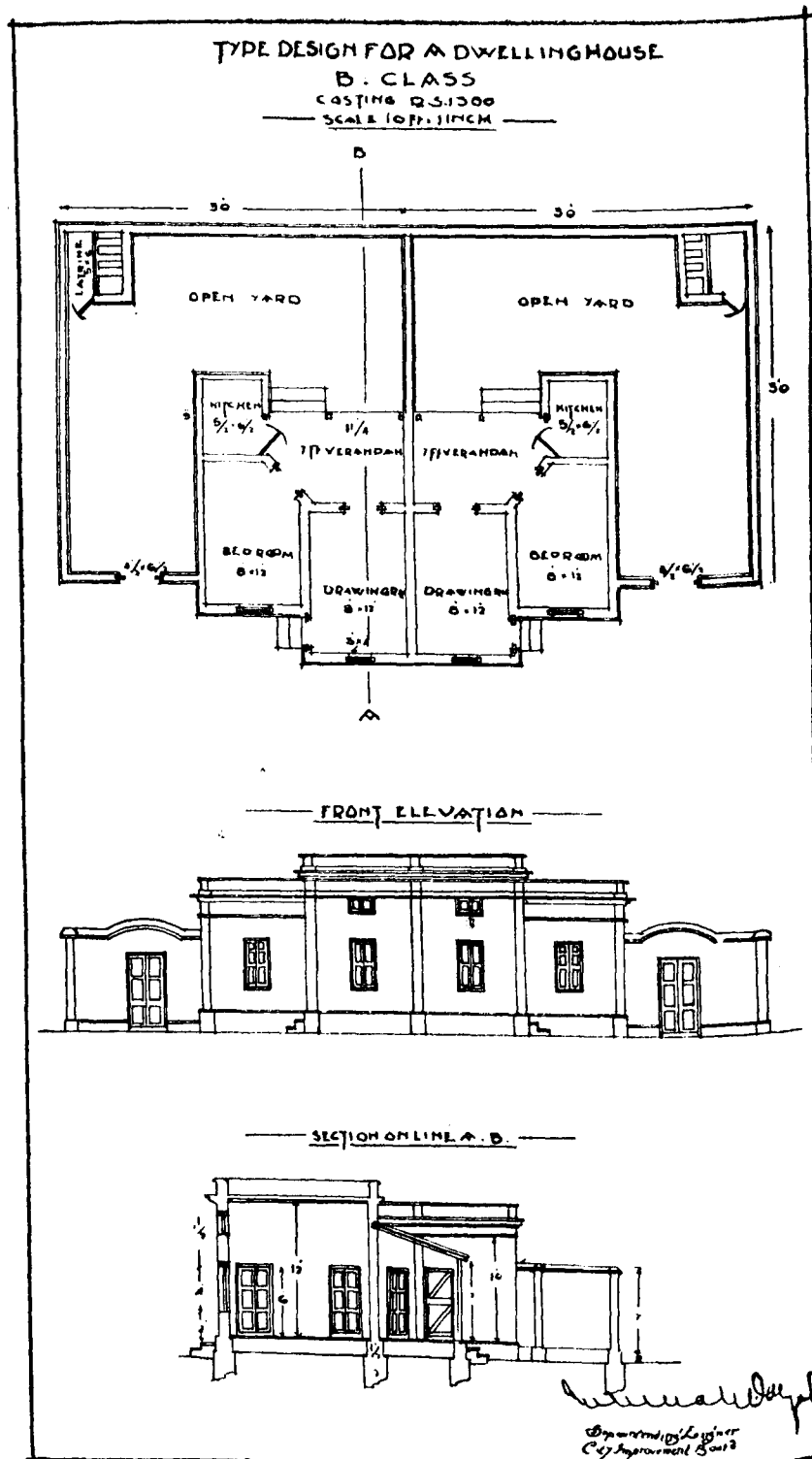
PLANS OF BUNGALOWS PROVIDED FOR PERSONS DISHOUSED DURING THE SLUM CLEARANCE.
