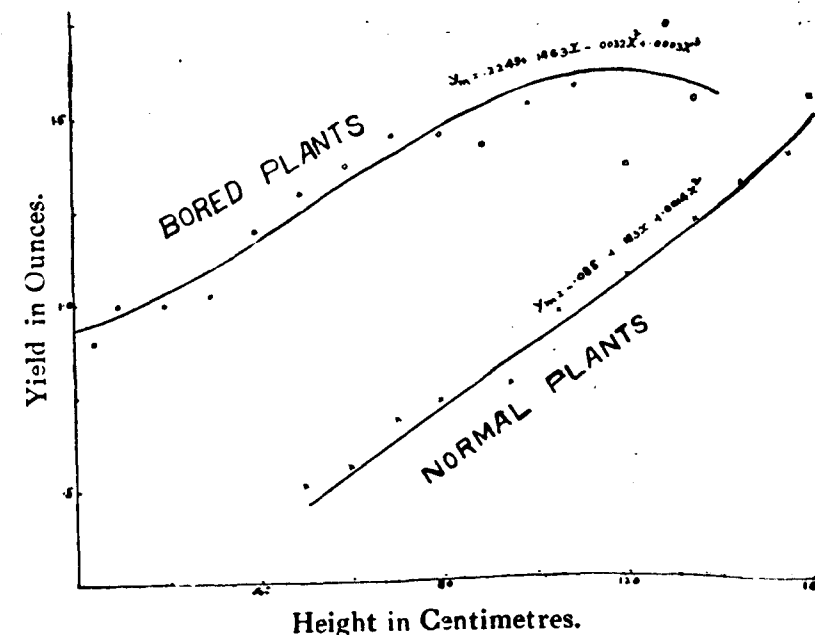
Fig. III. REGRESSION OF YIELD ON HEIGHT OF PLANT
