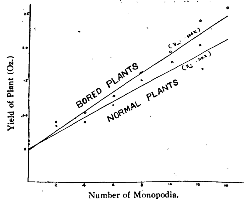
Fig. II. REGRESSION OF YIELD ON MONOPODIA
