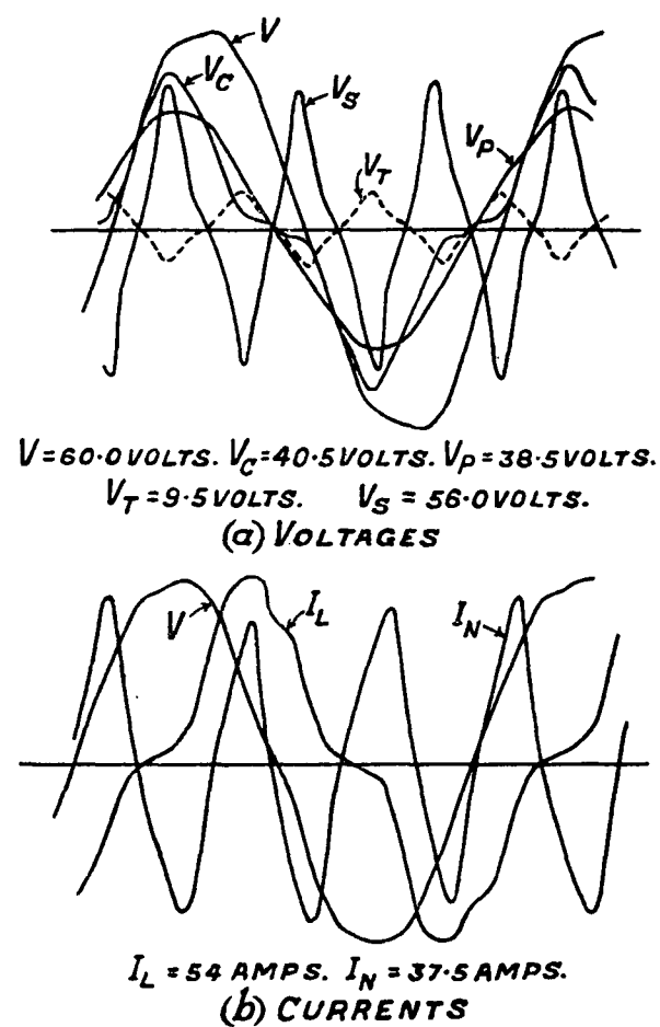
FIG. 13 STAR CONNECTION—NEUTRAL CONNECTED (4 TURNS IN TRANSFORMER)
