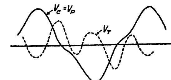
V_C = 36.75 \text{ VOLTS. } V_P = 36.75 \text{ VOLTS. } V_T = 1.00 \text{ VOLTS} (a) VOLTAGES
