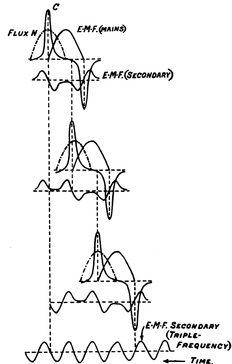
FIG. 3 PRINCIPLE OF COMBINING THREE PHASES TO FORM SINGLE PHASE TRIPLE FREQUENCY OUTPUT (TAYLOR'S ARRANGEMENT)
