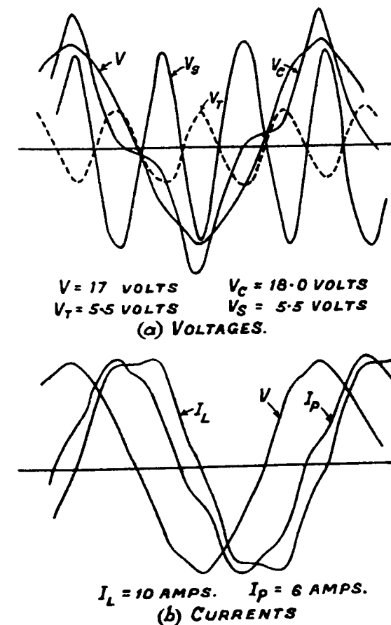
FIG. 8 DELTA CONNECTION
