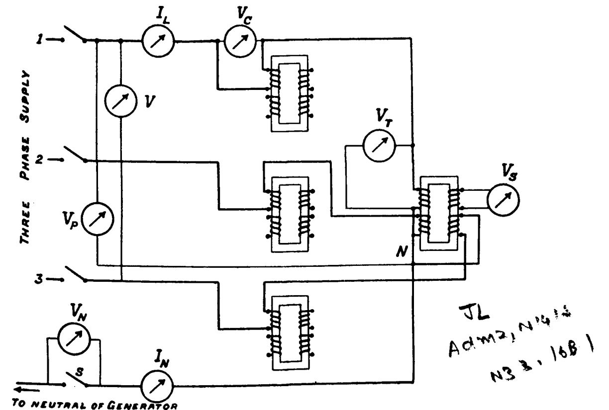
FIG. 10 DIAGRAM OF STAR CONNECTION
