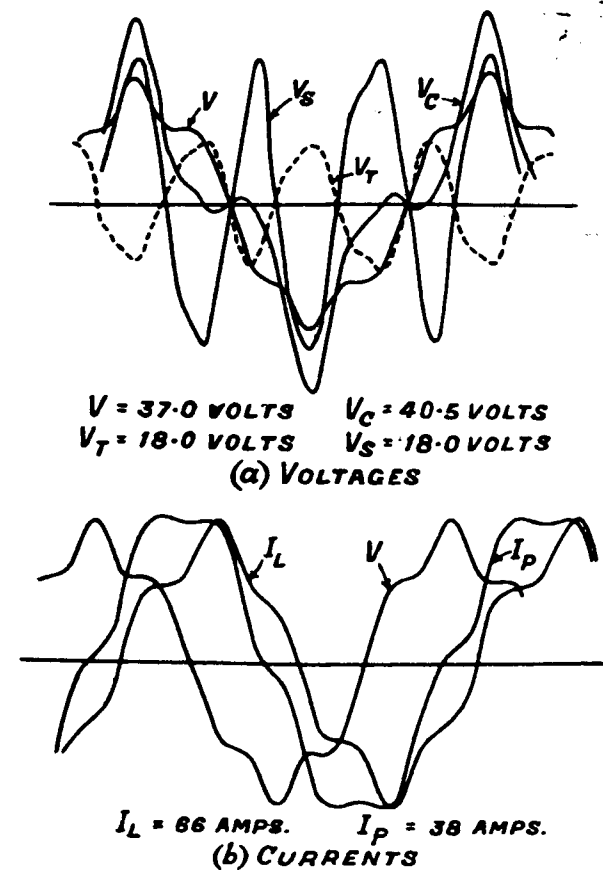
FIG. 9 DELTA CONNECTION
