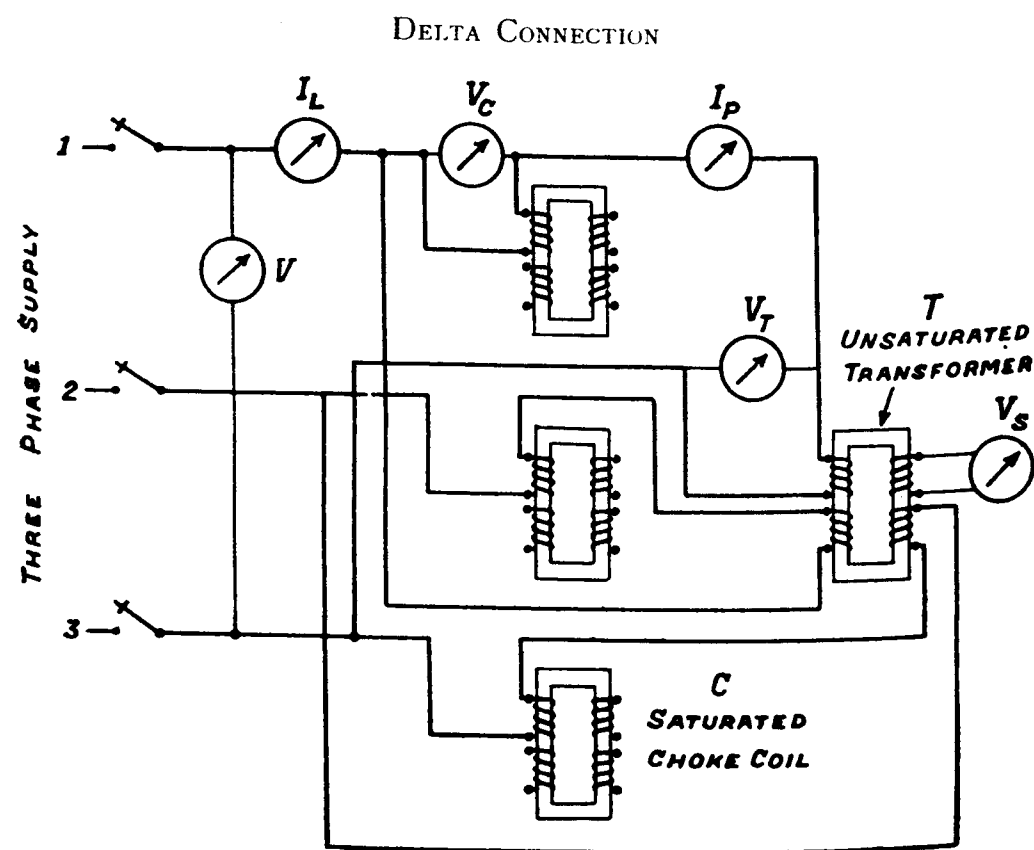
Fig. 7 shows the diagram of connections of the tripler which was supplied at 25 cycles from a 25/60 cycle, three-phase, 92/220 volt, 12.5/30 kW., sine-wave generator. Four similar 100/200 volt, 25 cycle, 10 kVA., core type, single-phase transformers each having
