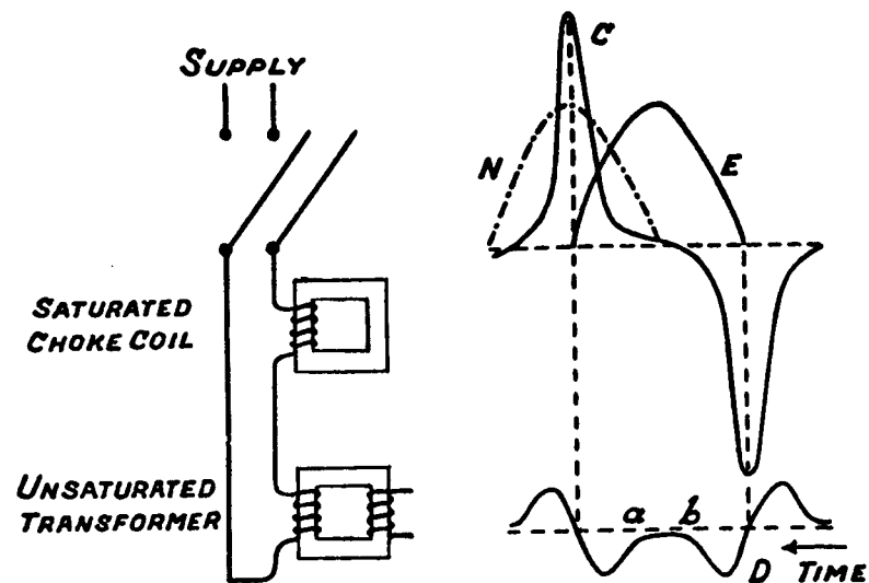
FIG. 2 PRINCIPLE OF TAYLOR'S ARRANGEMENT
