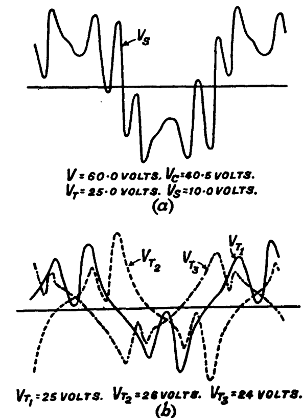
FIG. 14 DELTA CONNECTION—EFFECT OF LEAKAGE
