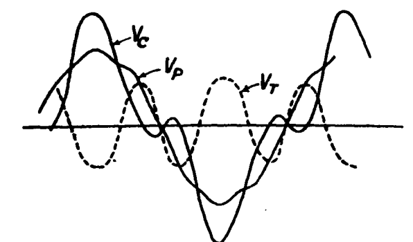
V_C = 40.5 \text{ VOLTS. } V_P = 37.0 \text{ VOLTS. } V_T = 16.0 \text{ VOLTS.} (a) VOLTAGES.
