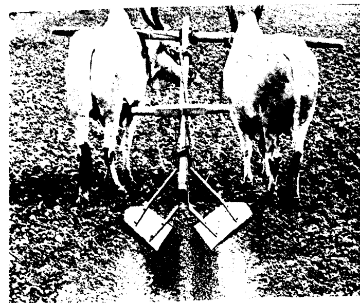
Bund former in operation showing compact and neatly shaped bund produced. Quality of work depends on soil tilth.
