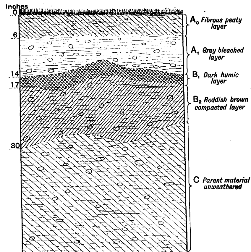
FIG. 1. — A PODSOL PROFILE.
