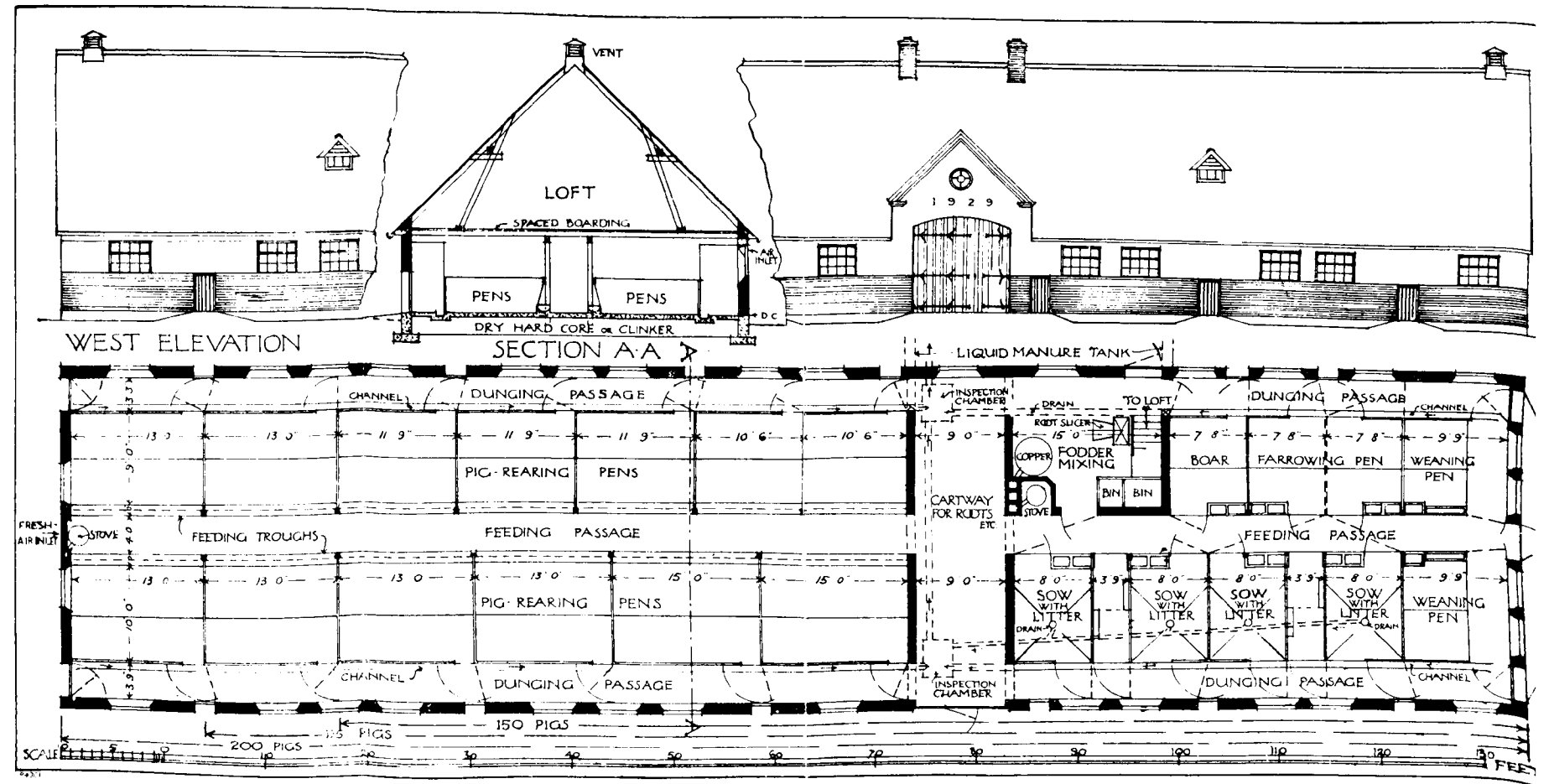
FIG. 1. Swedish type of pighouse. (For detail drawing see pages 696 and 697.)
