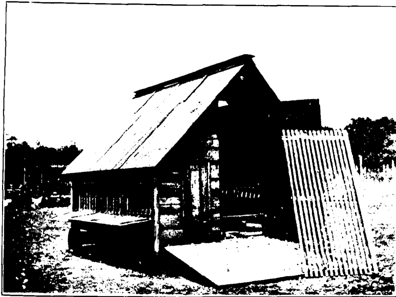
FIG. 3. Slatted floor house, showing detachable slatted floor, metal dropping-tray, and indoor and outdoor feeding.
