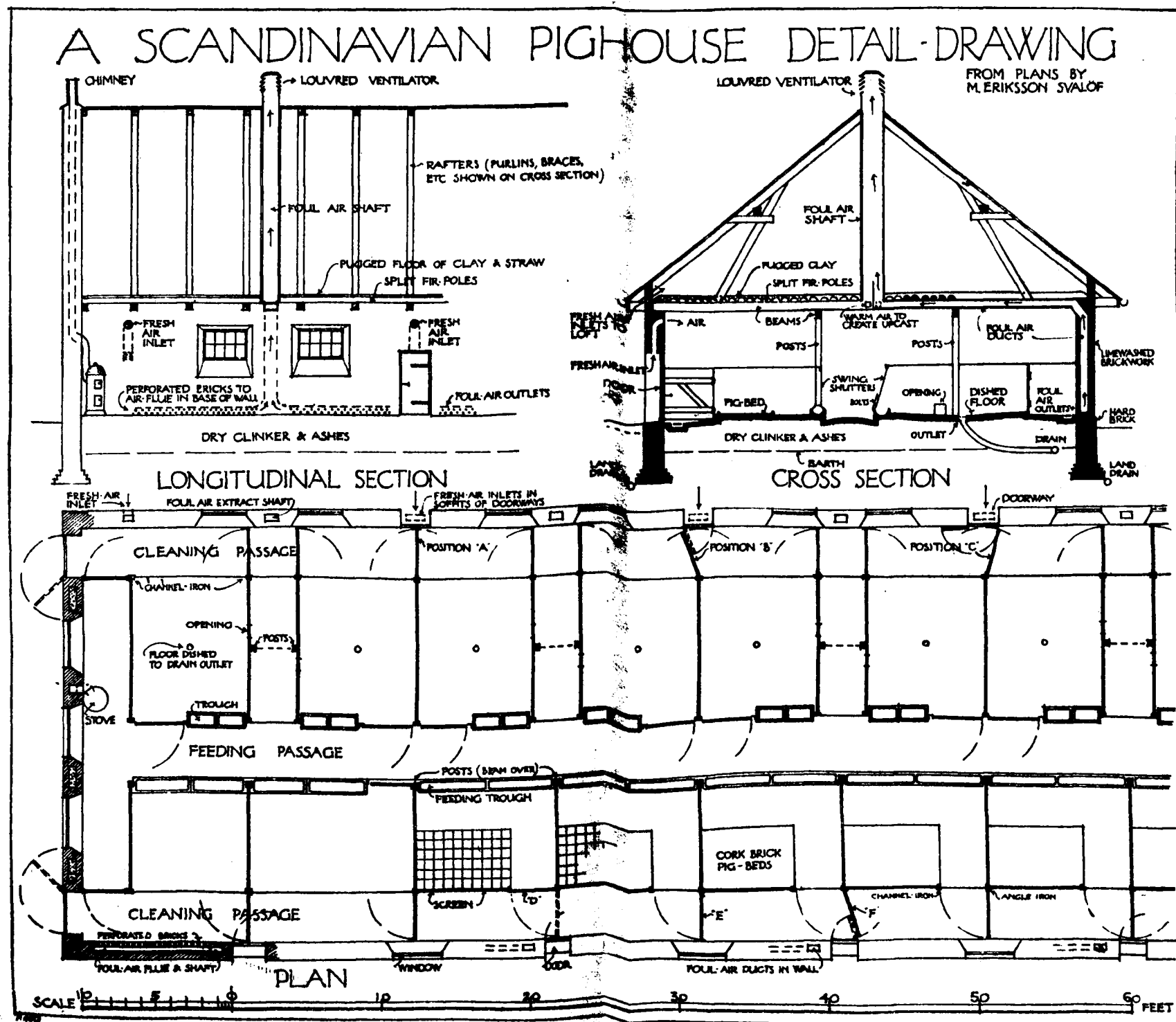
Fig. 2.—Details of Swedish type of pig-house shown in Fig. 1.
