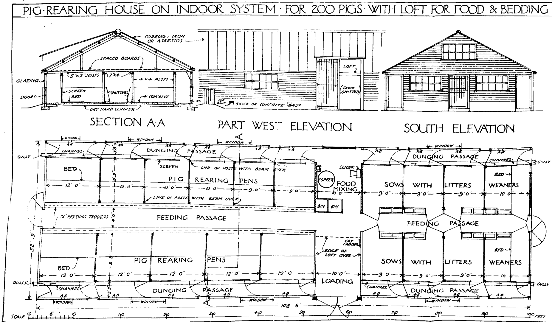
FIG. 6. Simplified form of Swedish pig house suitable for English climatic conditions.
