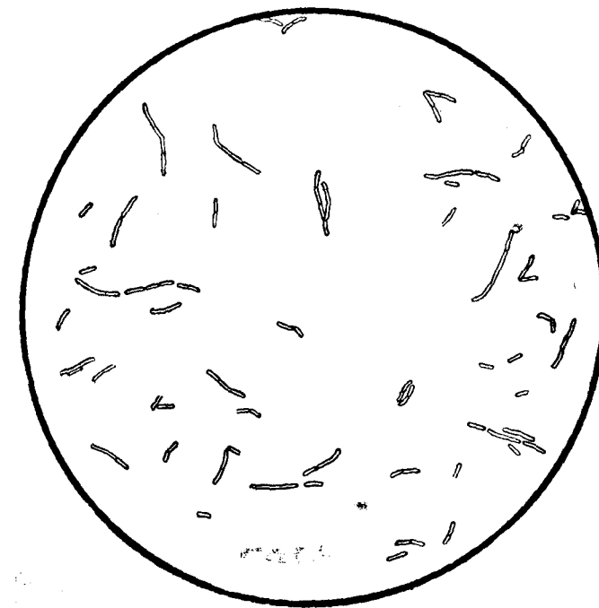
Fig. II Involution . Forms.
