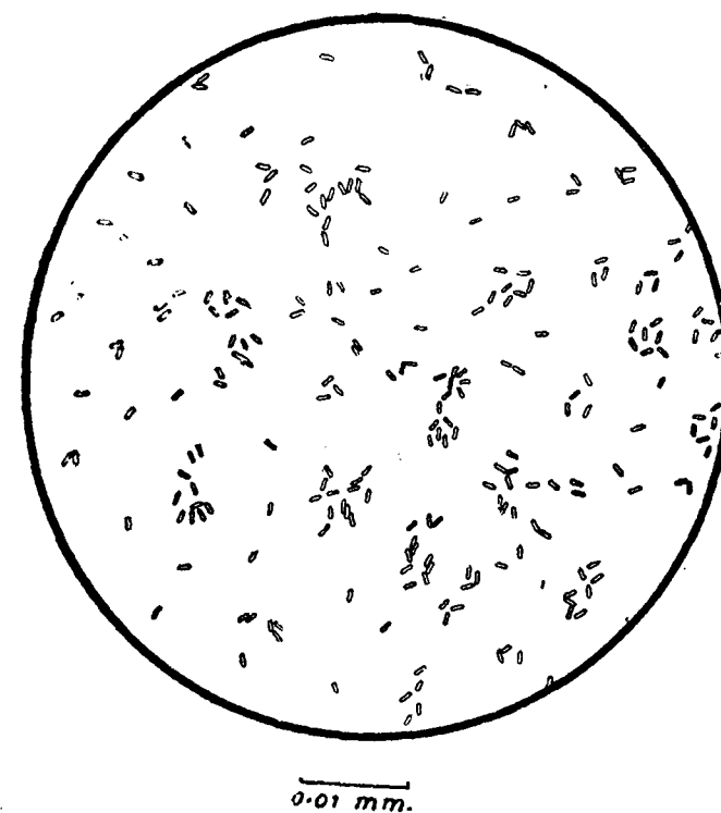
Fig. I Normal Forms
