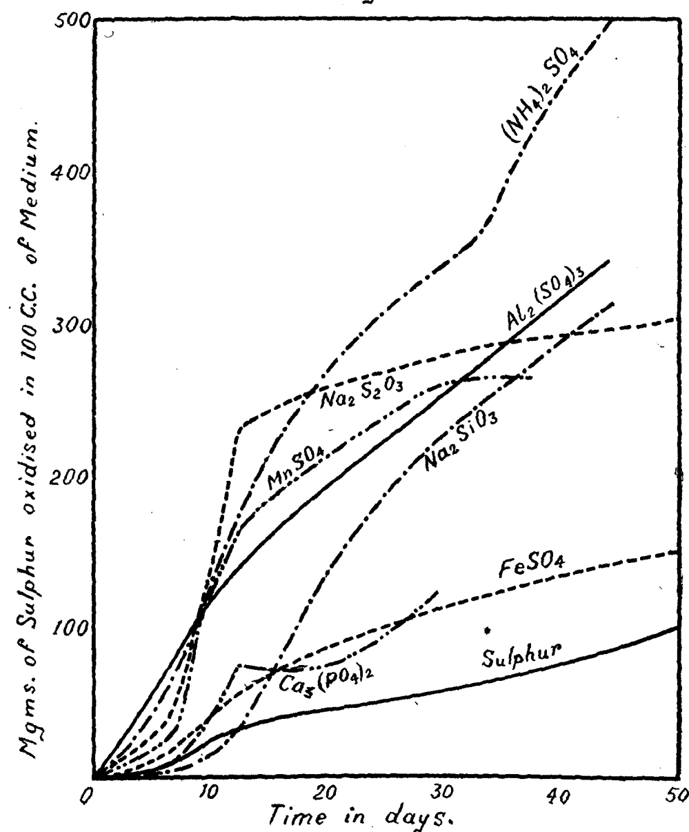
Fig. V Influence of inorganic salts.
