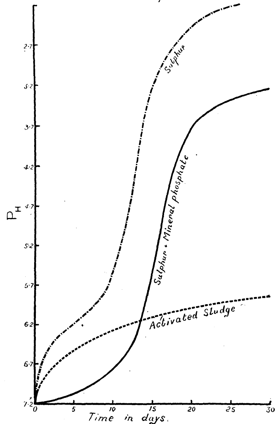
Fig. I P_H Changes during the Oxidation of Sulphur
