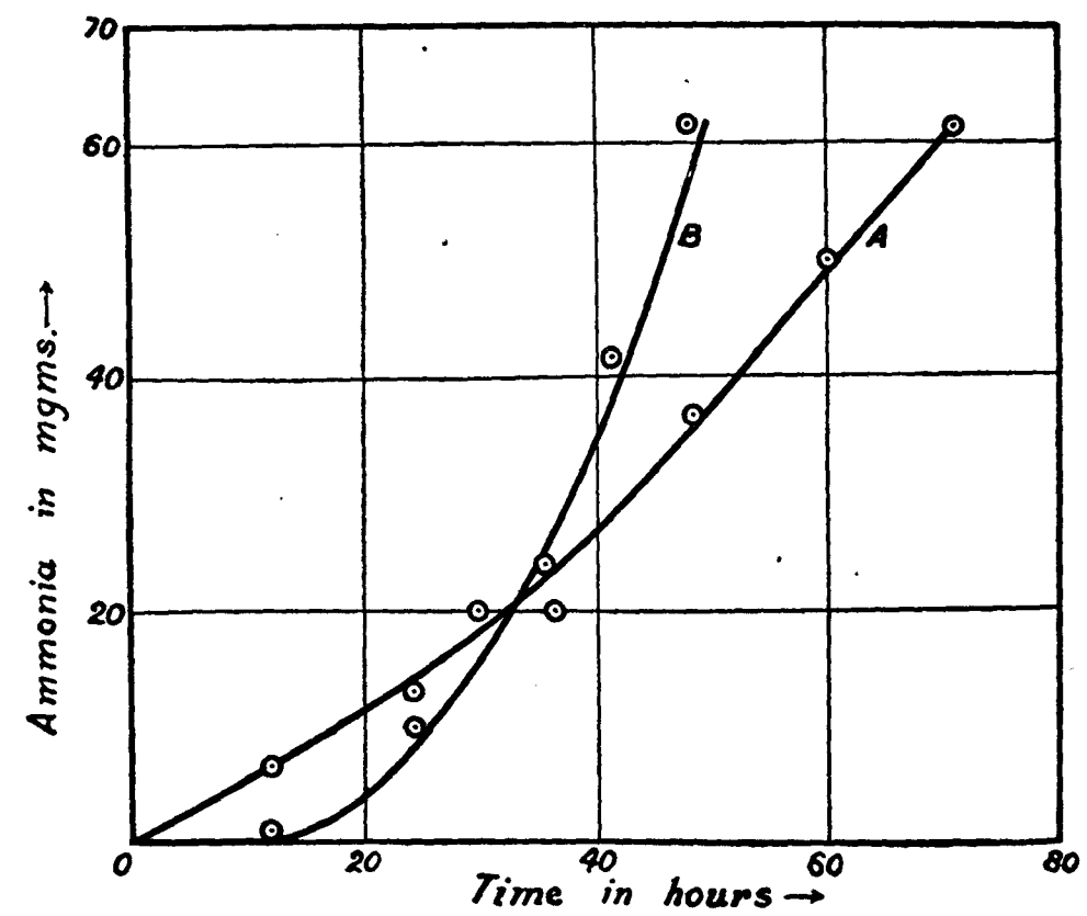
Fig. III. Influence of ammonia on the rate of reaction A : Ammonia B : Phosphates } P_H = 8
