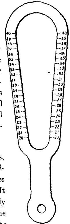
FIG. 2. Caliper (designed by E. C. Chilcott and L. J. Briggs) for measuring the diameter of cotton bolls without removing them from the plant. The angle formed by the diverging sides of the loop and the calibration of the intervals (millimeters) marked on them are so calculated that when the loop is placed horizontally over the boll at its point of greatest diameter and is pushed forward (from the handle) as far as possible without compressing the boll, the maximum diameter of the boll is indicated by the figure on the scale at the point with which the side of the boll is in contact.
