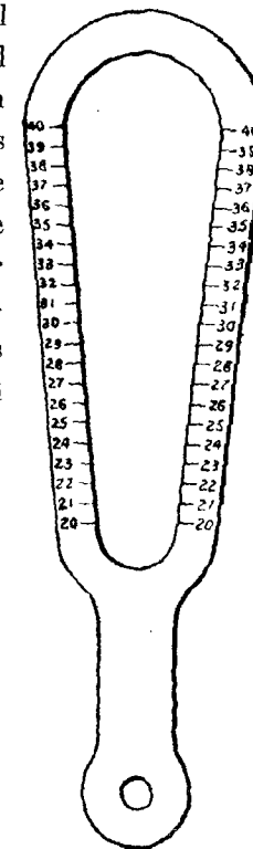
FIG. 2. Caliper (designed by E. C. Chleott and L. J. Briggs) for measuring the diameter of cotton bolls without removing them from the plant. The angle formed by the diverging sides of the loop and the calibration of the intervals (millimeters) marked on them are so calculated that when the loop is placed horizontally over the boll at its point of greatest diameter and is pushed forward (from the handle) as far as possible without compressing the boll, the maximum diameter of the boll is indicated by the figure on the scale at the point with which the side of the boll is in contact.
