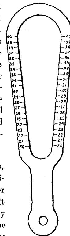
FIG. 2. Caliper (designed by E. C. Chilcott and L. J. Briggs) for measuring the diameter of cotton bolls without removing them from the plant. The angle formed by the diverging sides of the loop and the calibration of the intervals (millimeters) marked on them are so calculated that when the loop is placed horizontally over the boll at its point of greatest diameter and is pushed forward (from the handle) as far as possible without compressing the boll, the maximum diameter of the boll is indicated by the figure on the scale at the point with which the side of the boll is in contact.
