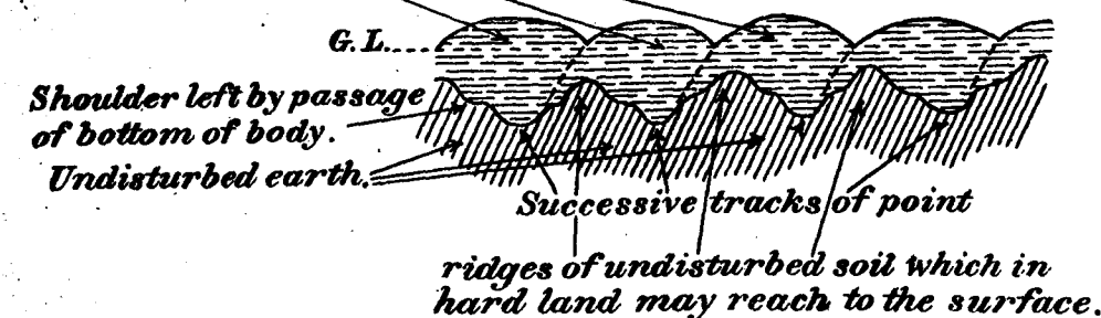
Diagrammatic representation of the work of a country plough.
