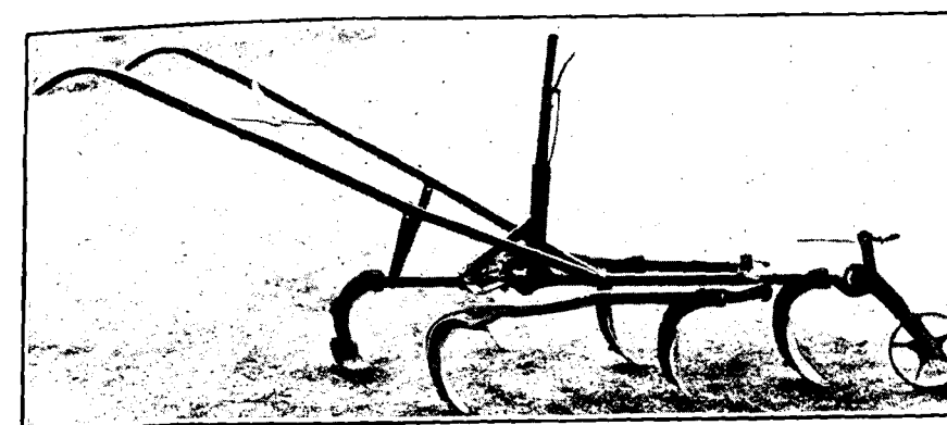
Fig. 2. Horse hoe for turning in the weeds and breaking the surface crust.
