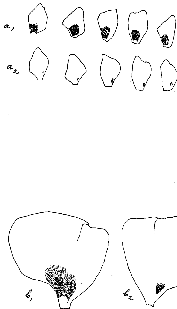
The petals. a 1 , ♀ 455 a (from the inner side); a 2 , ♀ 455 a (from the outer side); b 1 , ♀ 455 a × ♂ 59 (from the inner side); b 2 , ♀ 455 a × ♂ 59 (from the outer side).
