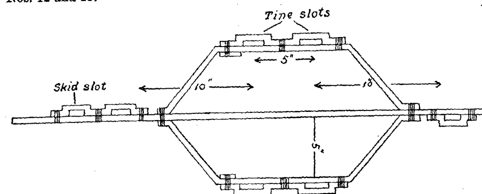
Fig. 12. Bihar 3-tined cultivator. Scale, 1'' = 7\frac{1}{2}'' .
