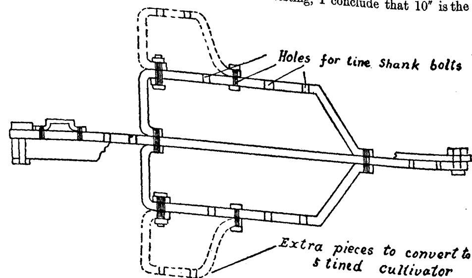
Fig. 14. The Bihar 3-5-tined cultivator. Scale, 1" = 7½".
