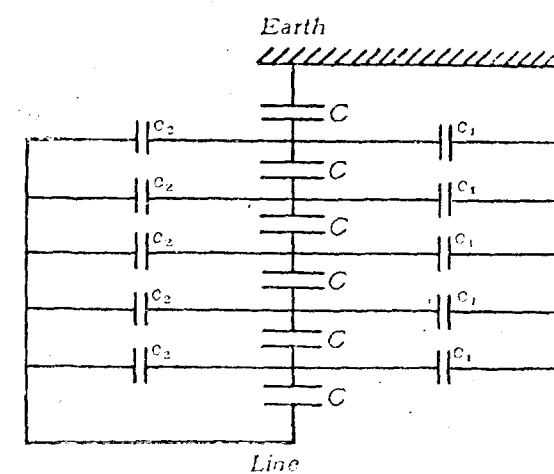
Fig. 1. Equivalent Circuit
