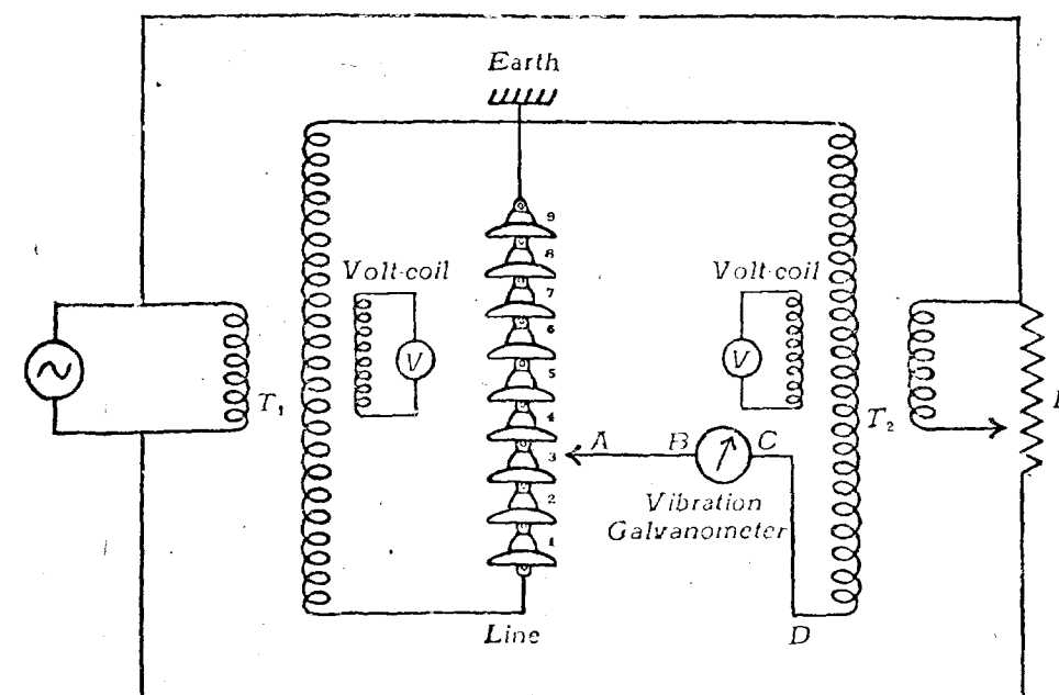
Fig. 2. Auxiliary Transformer Test Circuit
