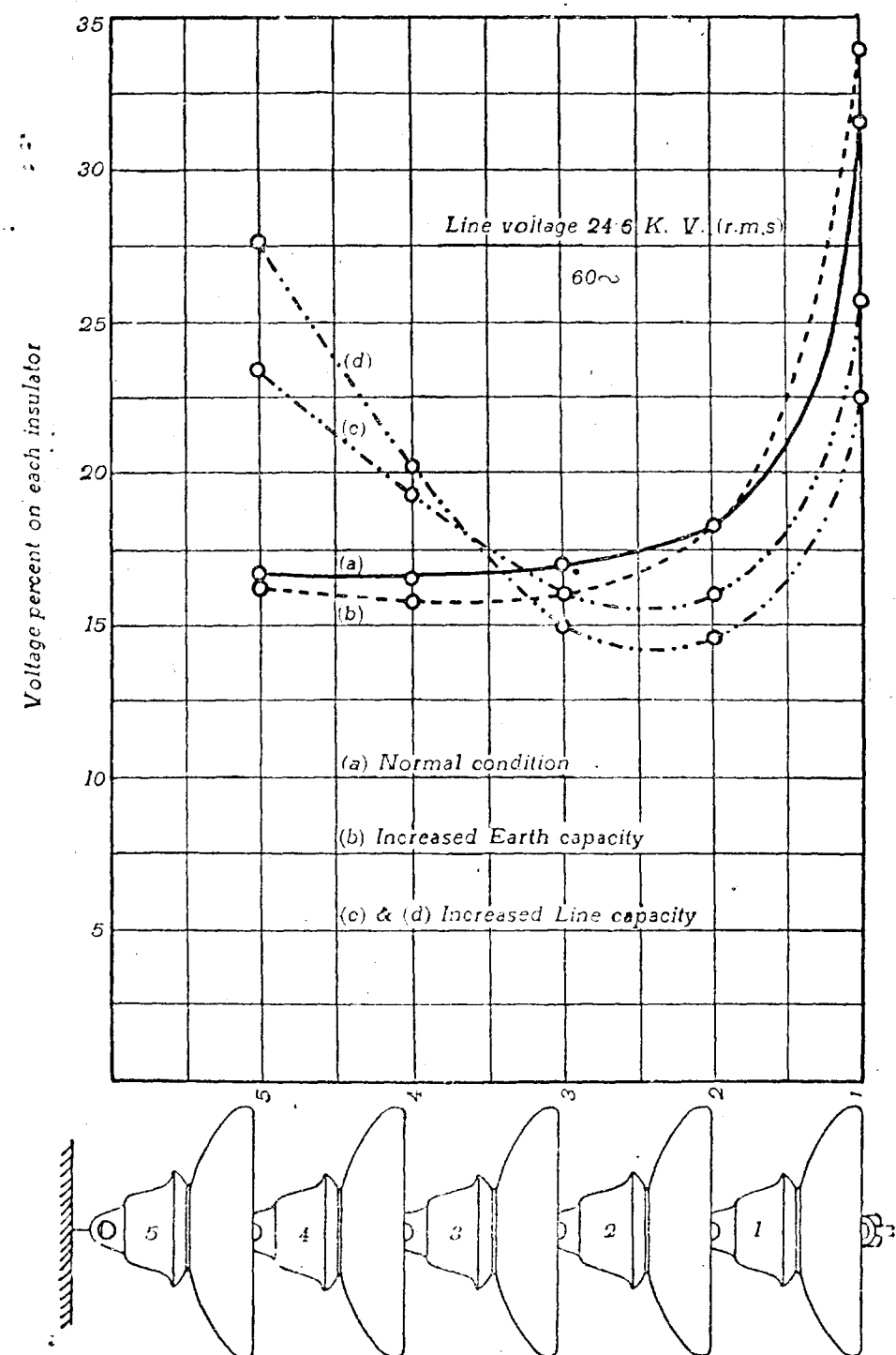
Fig. 5. Effect of Earth and line capacities on the voltage gradient
