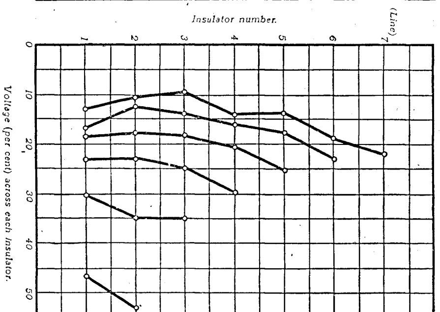
Fig. 5. Auxiliary transformer method and old Insulators.
