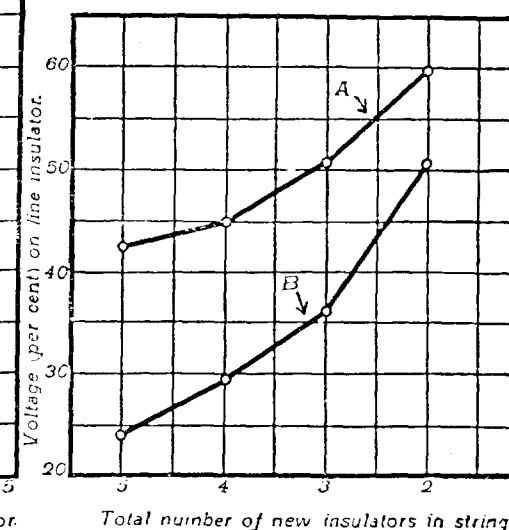
Fig. 2. Variation of line-unit voltage.
