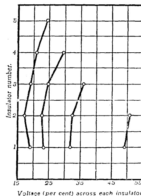
Fig. 6. Auxiliary transformer method and new insulators.
