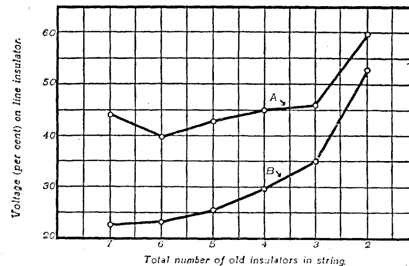
Fig. 1. Variation of line-unit voltage.
