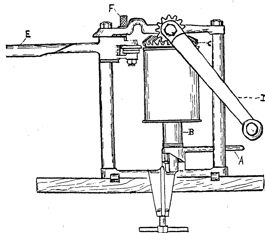
FIG. 4.—Diagram of Hand Power Can-Sealing Machine, with Can in position for Sealing.
