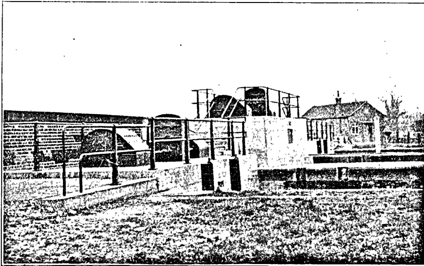
FIG. 9.—Middle Level Sluices, St. Germain. View of control gear.
