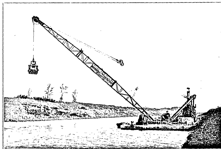
FIG. 7.—Middle Level. Another view of dredger showing large working radius.
