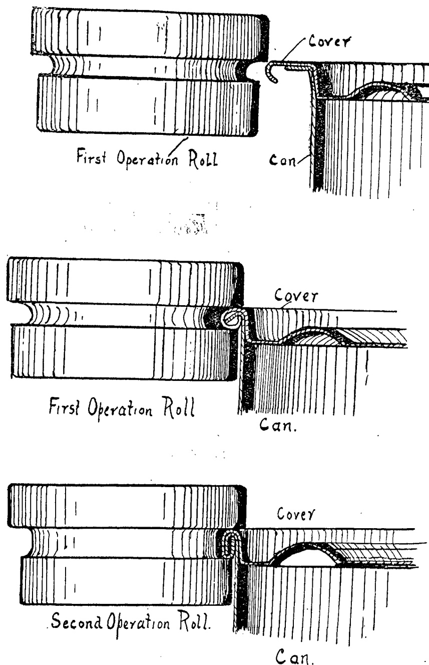
FIG. 5.—Top, Position of 1st operation roller. „ 6.—Centre, Can and Lid after the 1st operation. „ 7.—Bottom, Completion of Sealing the Can.
