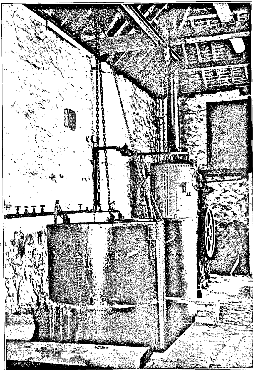
FIG. 3.—Bulb-Treating Plant. Scilly Experimental Station.
