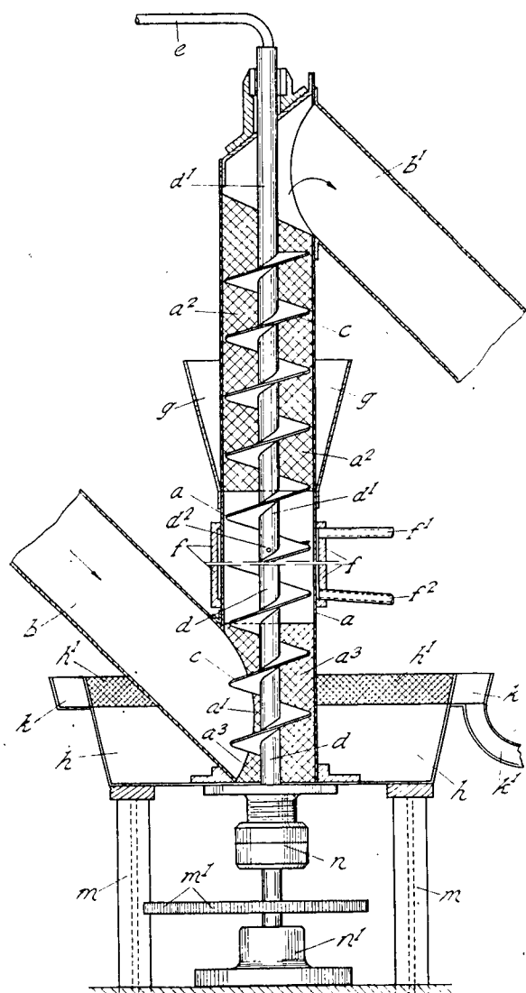
FIG. 4.—Continuous Diffuser Extractor.
