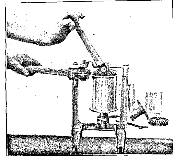
FIG. 1.—Hand Power Can-Sealing Machine.
