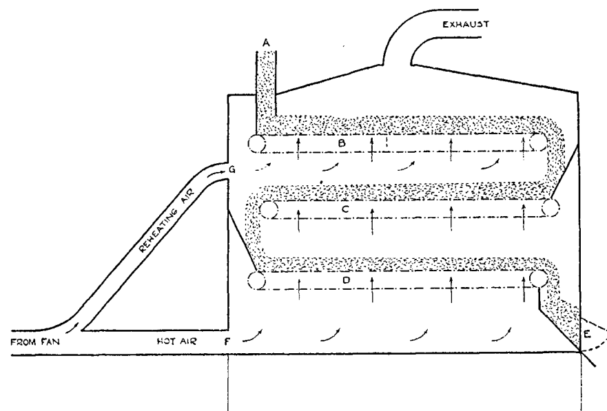
FIG. 1.—Continuous Mass Drying for Factory or Farm.
