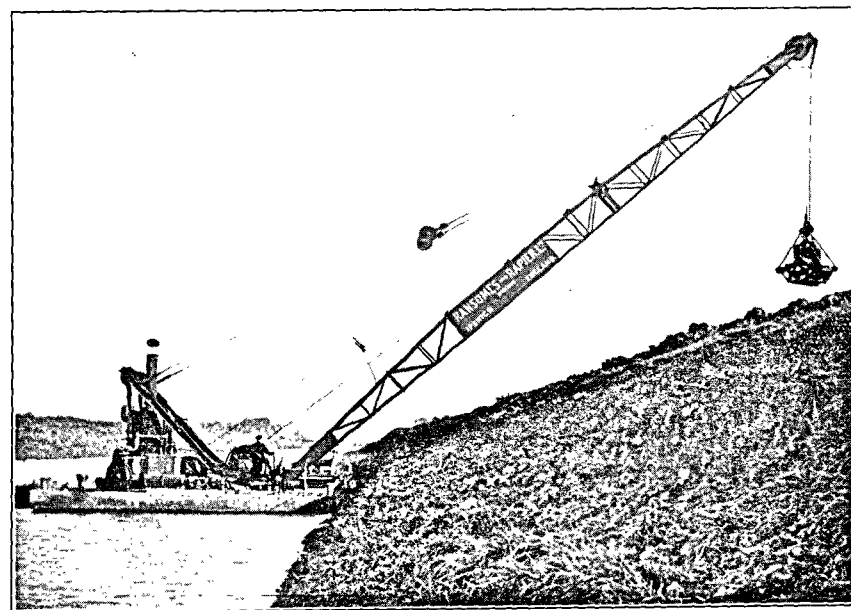
FIG. 6.—Middle Level. New dredger at work on main drain.
