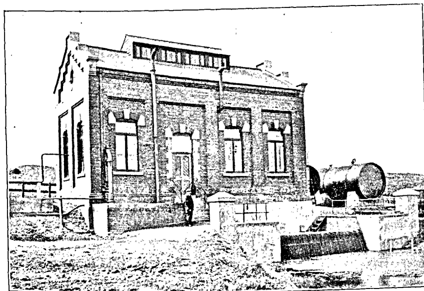
FIG. 2.—Littleport and Downham Fen. View of new pump house showing drainage sump.
